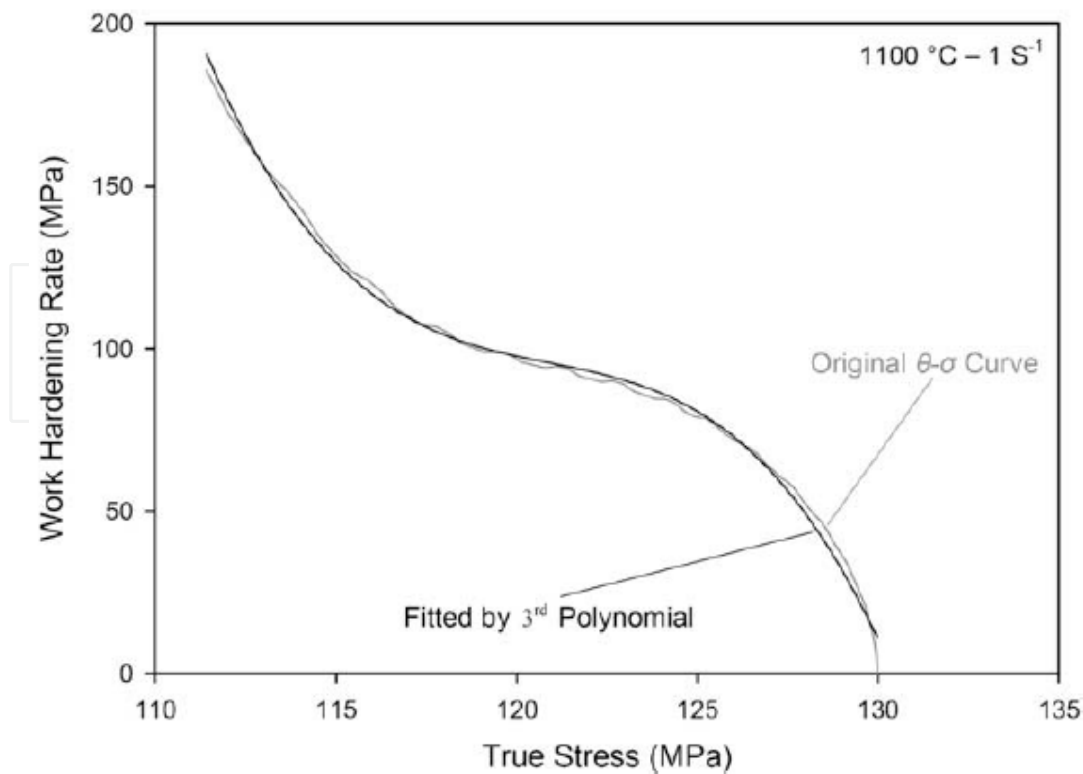
Fig. 6. The \theta - \sigma curve of 17-4 PH Stainless steel and its corresponding third order polynomial.
