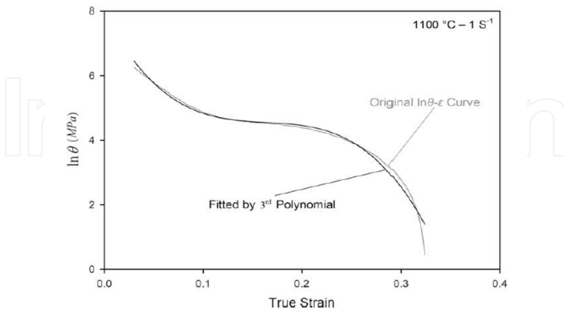
Fig. 8. The \ln\Theta-\epsilon curve for 17-4 PH stainless steel and its corresponding third order polynomial.
