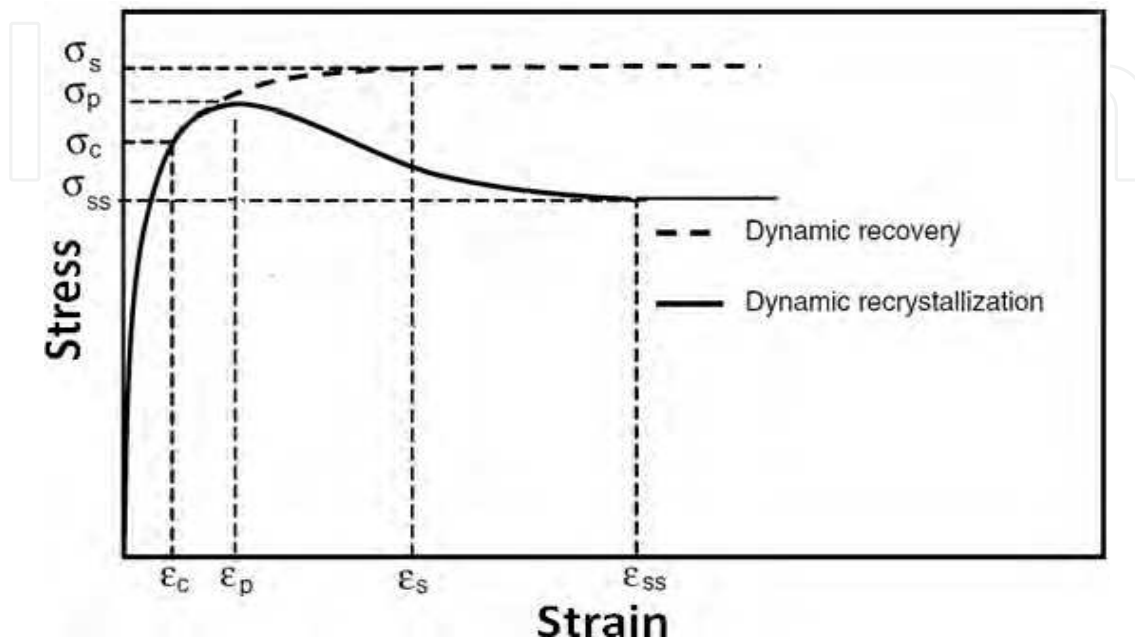
Fig. 4. Schematic representing of DRV and DRX.
