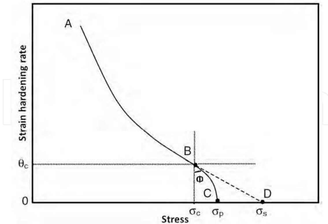
Fig. 5. Changes in the slope of the stress-strain curve with stress.
