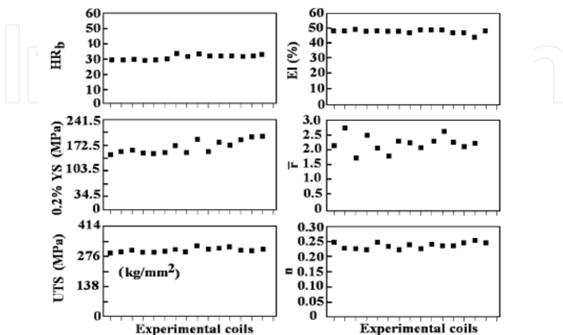
Fig. 13. Mechanical properties of annealed coils. (a) Hardness Rockwell b, (HRb), (b) 0.2% of yield strength, (YS), (c) tensile strength, (TS), (d) percent of elongation, (EI), (e) the average plastic anisotropy value, ( \bar{r} ) and (f) the strengthening hardening exponent, n (Mendoza et al., 2004).
