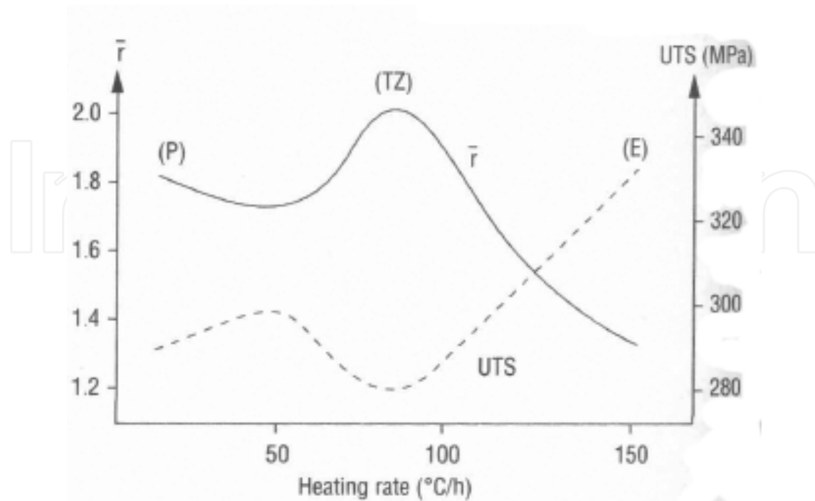
Fig. 5. Variation in \bar{r}_m UTS values and microstructure with heating rate for batch annealed aluminium killed steel (Beranger et al., 1996).
