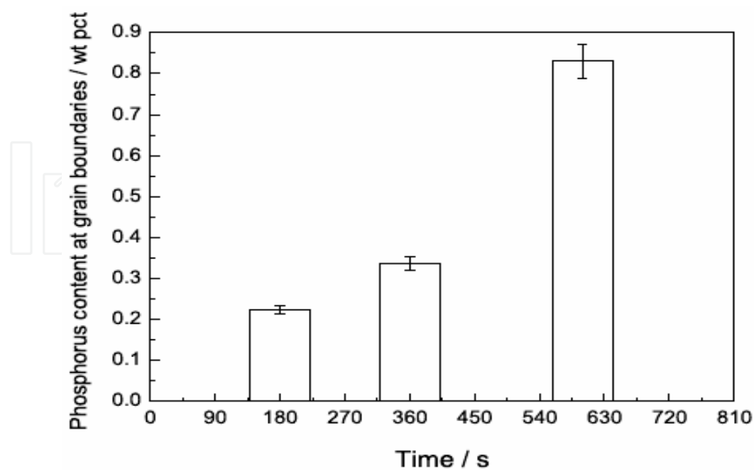
Fig. 29. Phosphorus content at grain boundaries in the rephosphorised IF steels annealed for different time 5 (Song, et al., 2010)
