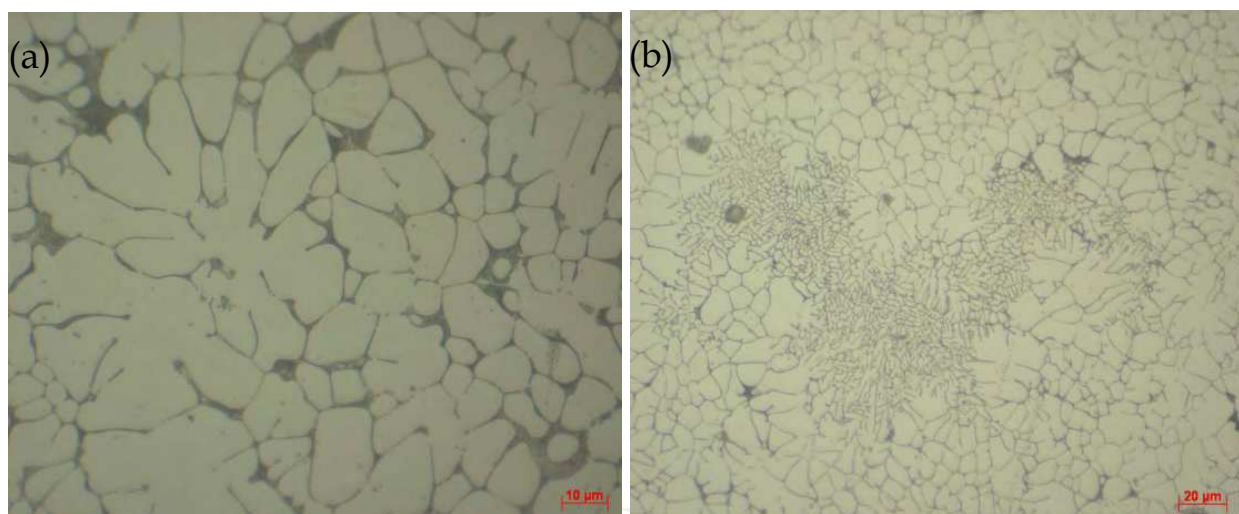
Fig. 18. Optical metallographs of AA8011 alloy. (a) die casting sample and (b) central region in 2 mm diameter sample in suction casting.
