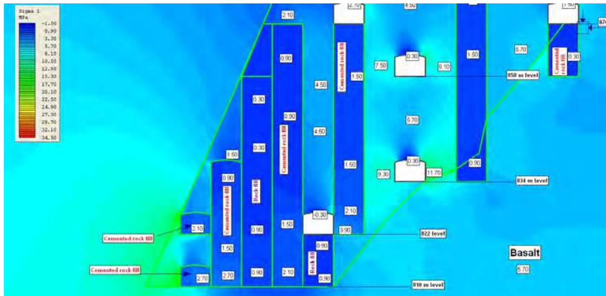
Fig. 5. Vertical stresses between 810 m level and 858 m level at west sector of mine.
