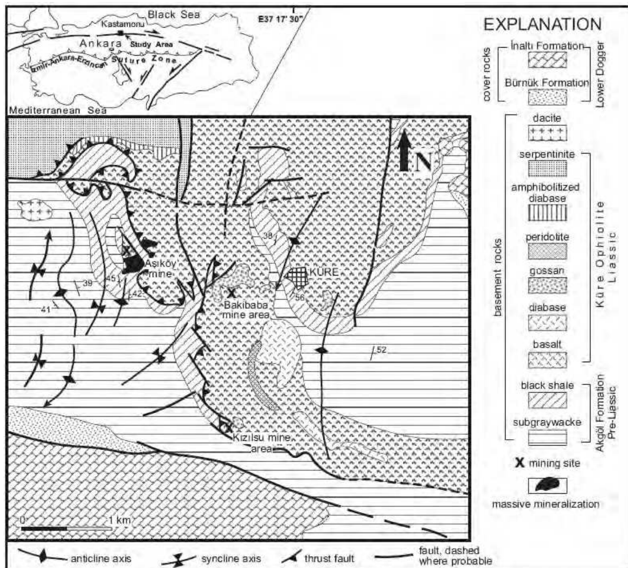
Fig. 1. Simplified geological map of the Küre mining district (Kuşçu and Erler, 2002) [3].
