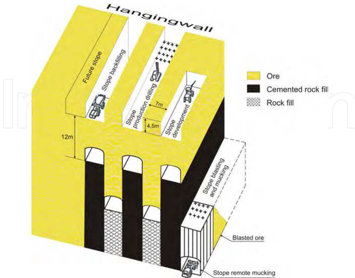
Fig. 4. Development, production and backfilling operations.
