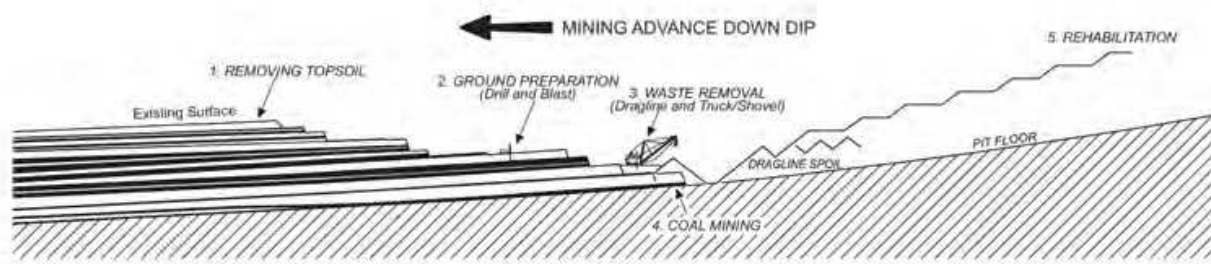
Fig. 3. Overall mining sequence of a typical surface coal mine in Australia (after Westcott et al., 2009).
