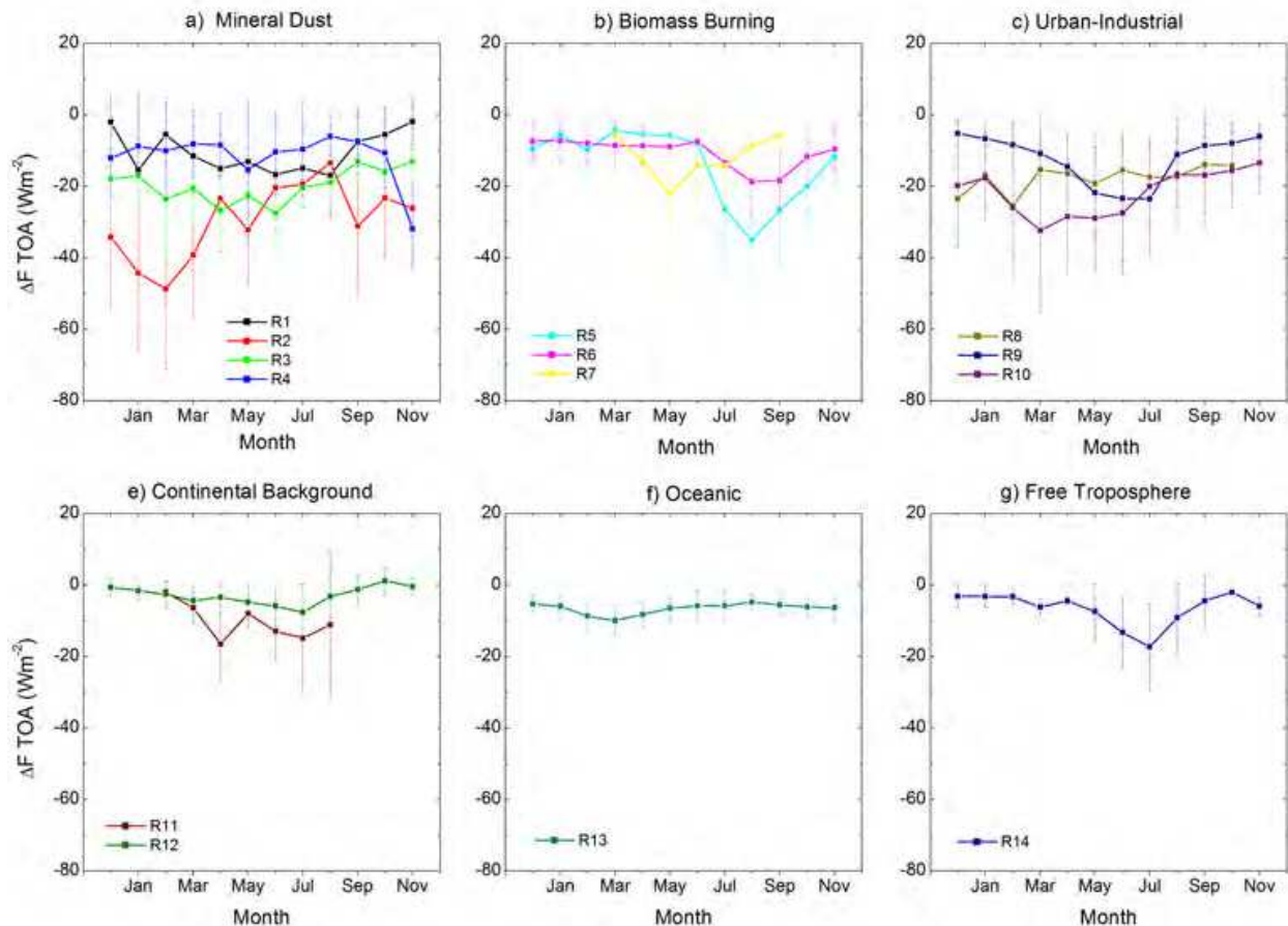
Fig. 10. Annual cycle of the inter-annual average of the aerosol radiative forcing ( \Delta F , \text{Wm}^{-2} ) at the TOA for the key aerosol types grouped into 14 regions and for surface reflectivity \text{SR} \leq 30\% . Error bars indicate 1\sigma (standard deviation).
