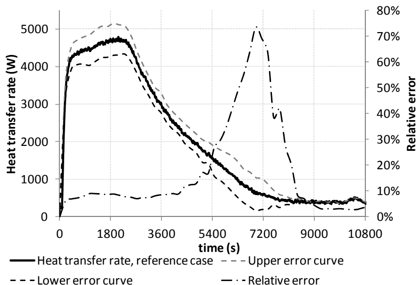
Fig. 11. Simulated heat rate, uncertainty bands and relative error (melting stage).
