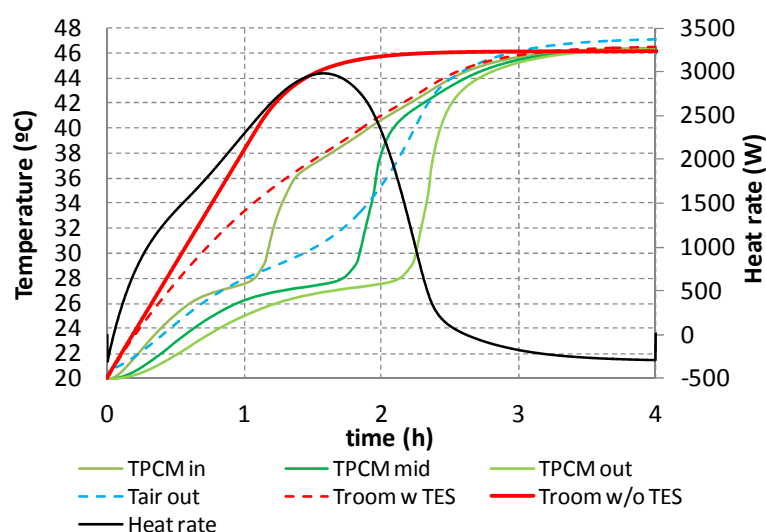
Fig. 14. Theoretical model simulated results of Lazaro's case (2009).
