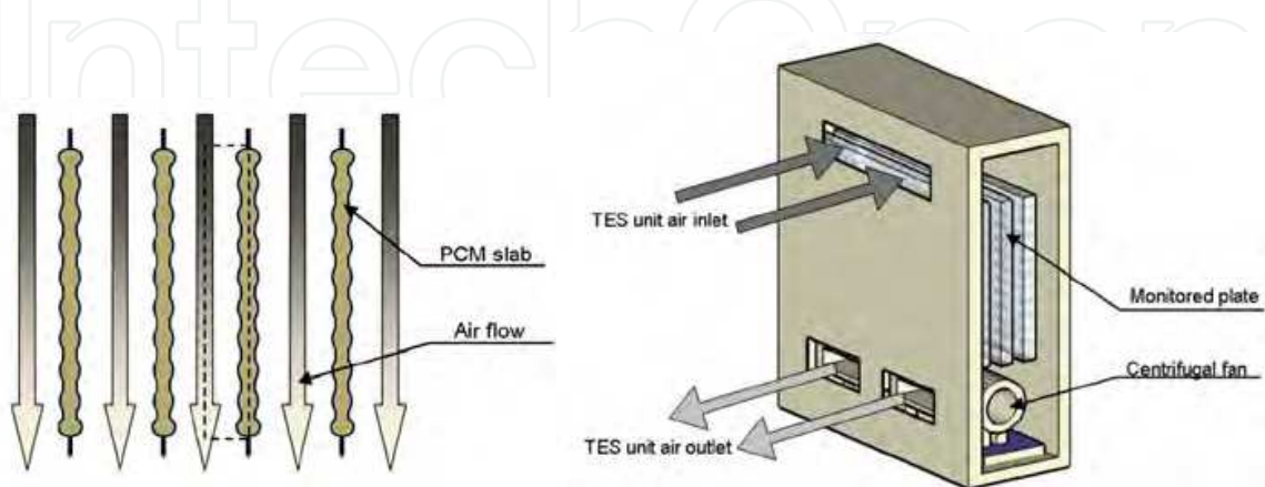
Fig. 5. PCM panels and air flow system (left); PCM-air heat exchanger (right).
