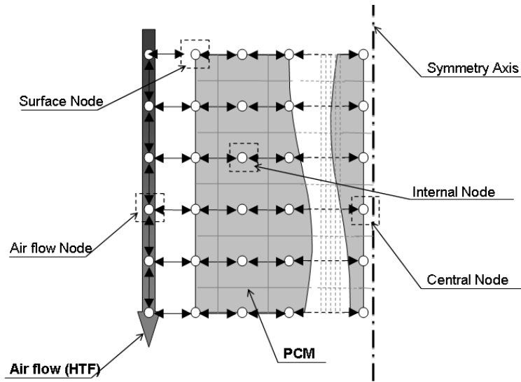
Fig. 10. Nodal distribution in the 1D plate system.
