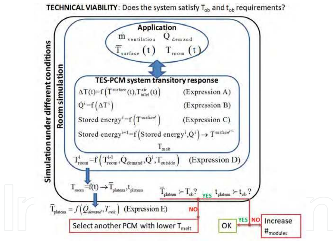
Fig. 9. Flow diagram to evaluate the technical feasibility of the system (Lazaro et al., 2009b).
