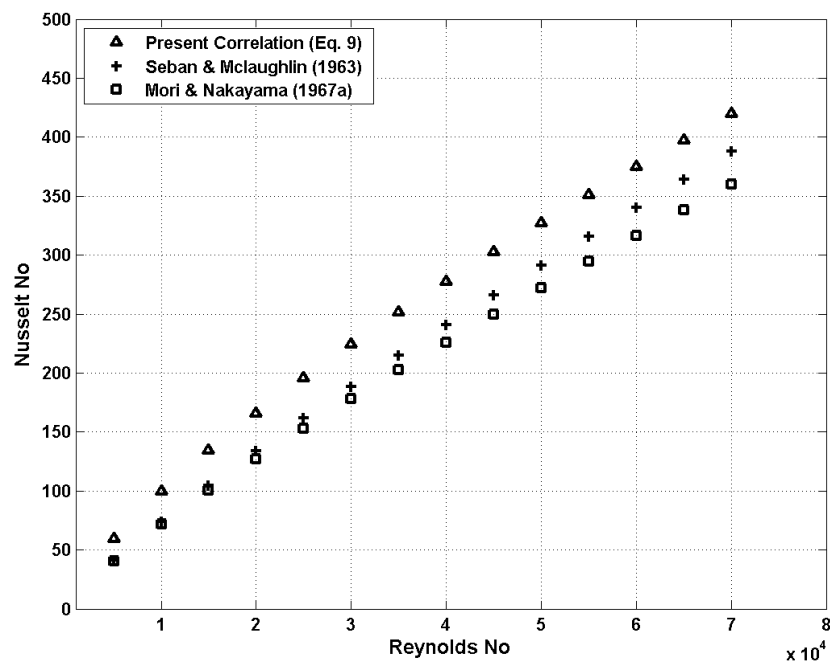
Fig. 9. Comparison of Nusselt number for the constant wall flux B.C.
