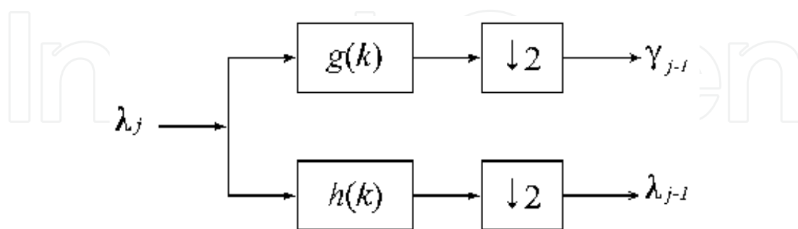
Fig. 5. Implementation of (23) and (24) as one stage of an iterated filter bank.
