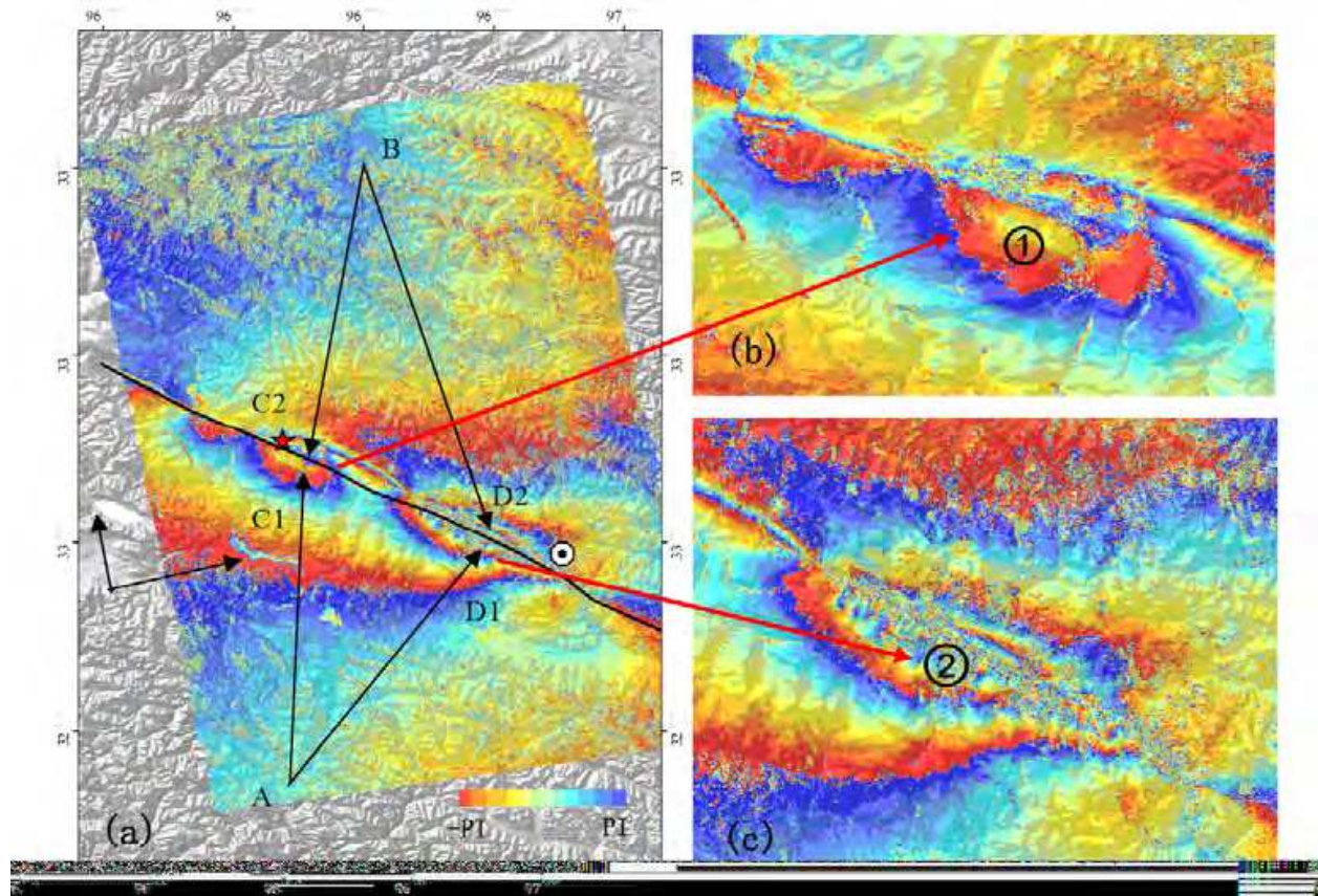
Fig. 5. Coseismic deformation map from ALOS PALSAR data, (a) Differential interferometric phase map; (b) Differential interferometric phase of instrumental epicenter; (c) differential interferometric phase of macro epicenter. A, B, C1, C2, D1 and D2 in (a) represent the different positions and in (b) and in (c) are two large deformation areas (from Guo et al., 2010b).
