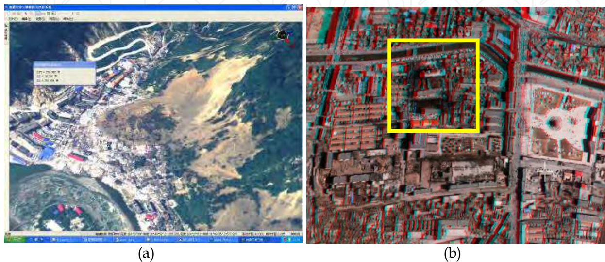
Fig. 8. (a) 3D analysis of secondary geological disasters in the Wenchuan earthquake, (b) 3D view in red-blue mode for damaged building extraction.
