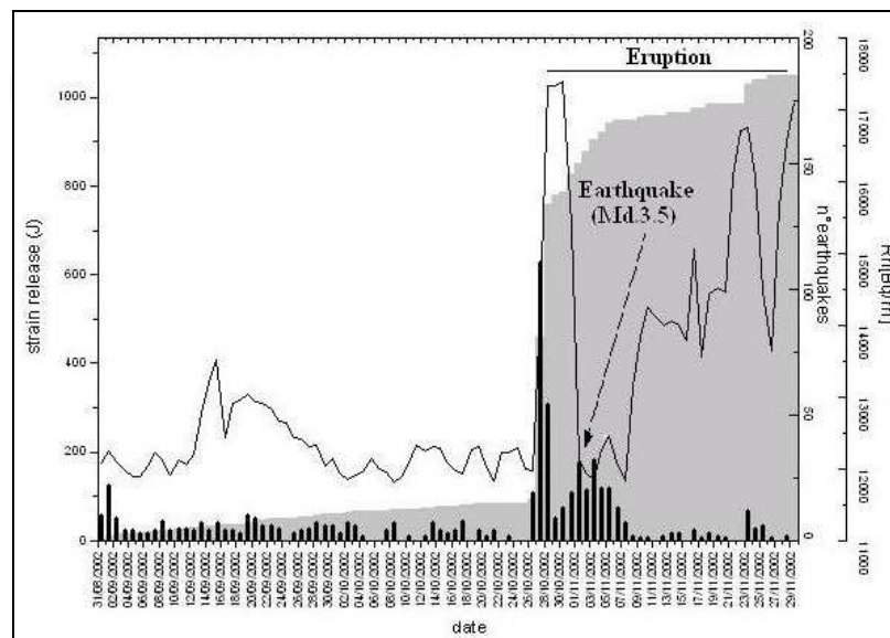
Fig. 3. Radon concentration (black line), daily earthquakes rate (black column bar) and strain release (grey histogram) measured in the period between 1 st September 2002 and 30 th November 2002 (Vena station). [Immè et al. , 2005]
