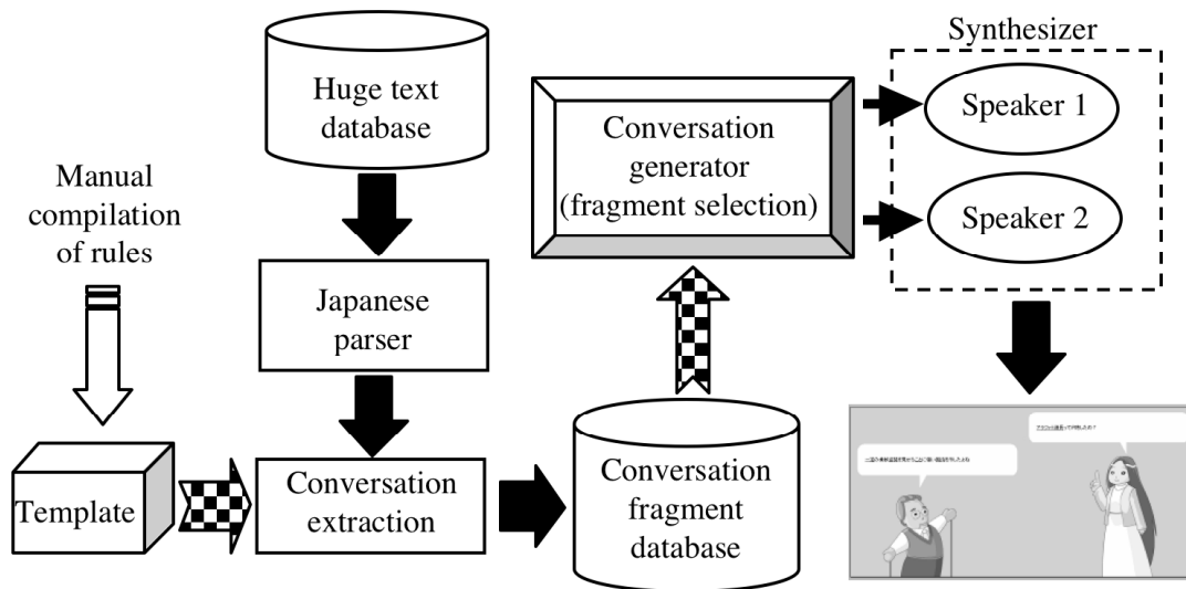
Fig. 2. System Flow of Sophisticated Eliza
