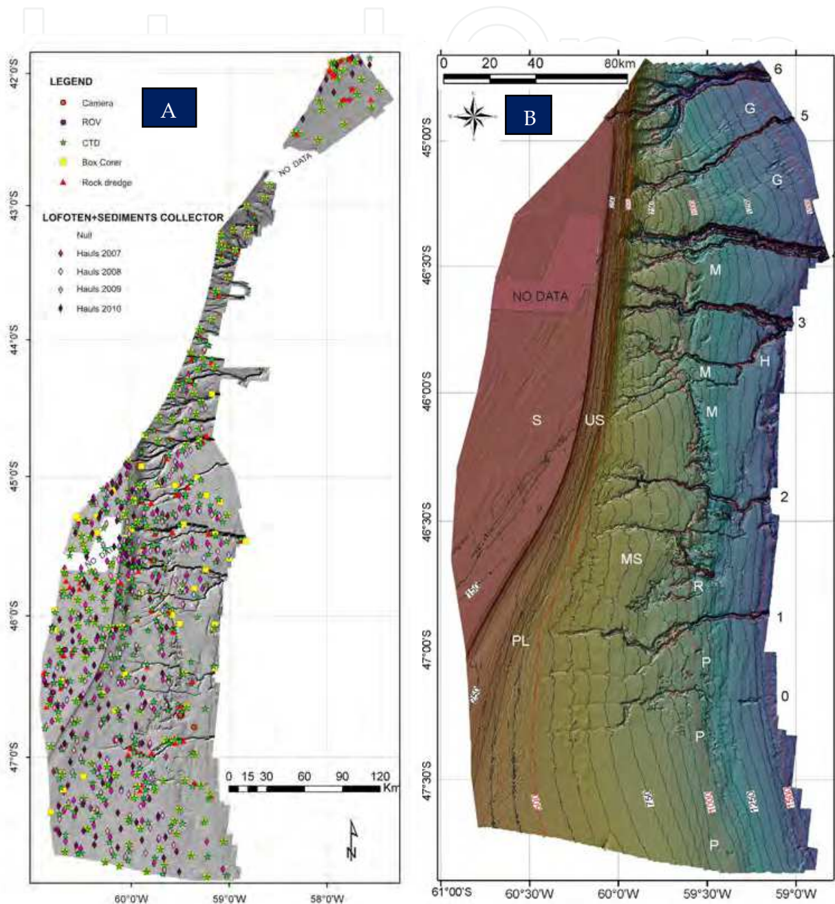
Fig. 1. A) Study area with the swath-mapped region and location of the different stations. B) Outer continental shelf and slope from 45°S to 48°S (southern region). G: gullies; M: moats; MS: middle continental slope; P: pockmarks; PL: iceberg plough marks; R: ridge; S: continental shelf; US: upper continental slope
