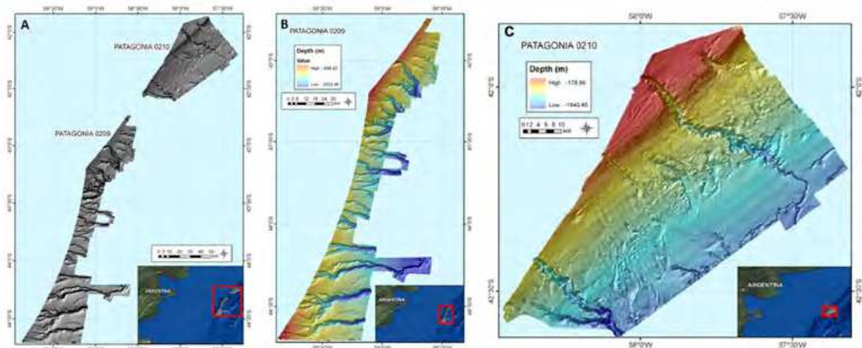
Fig. 2. A) Upper and middle continental slope between 41^{\circ}30'S and 45^{\circ}S (northern region) studied in 2009 ( B) and 2010 ( C)
