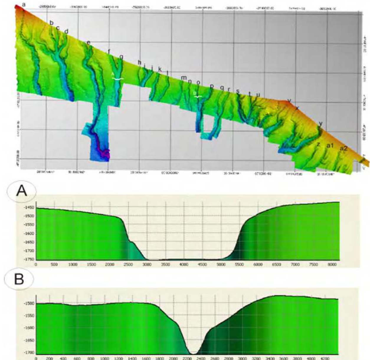
Fig. 5. Color coded DTM of Patagonia 02/09 area (landscape representation). a-y = Canyons. Lower panel A-B = Bathymetric cross section of f/g and o canyons. Note the different cross section in U and V
