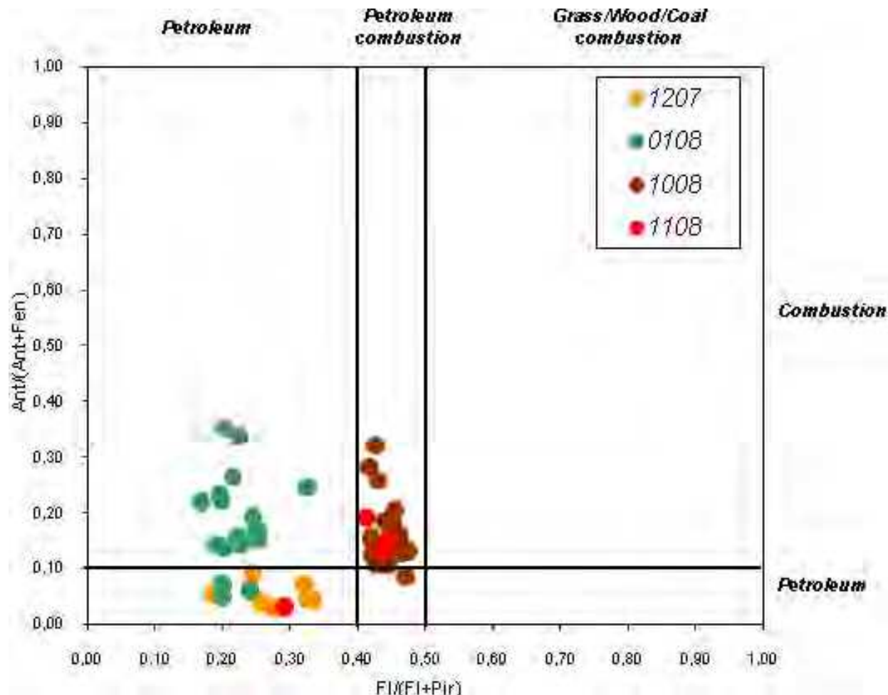
Fig. 16. Isomer ratios to identify PAH sources
