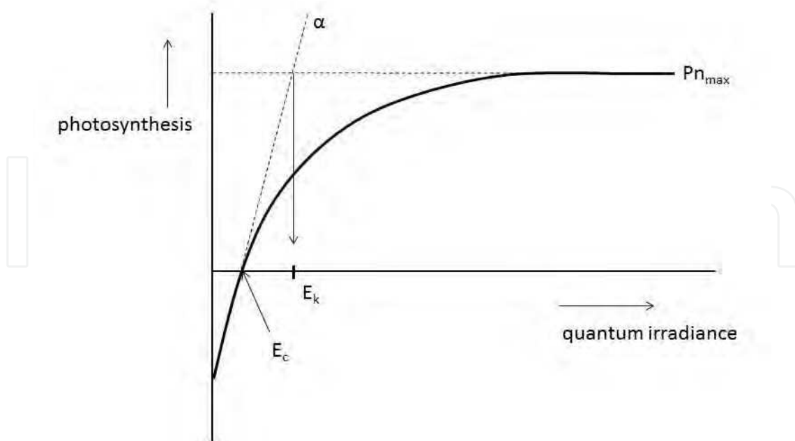
Fig. 3. Example of a curve that relates net photosynthesis to irradiance, showing the compensation point E_c , the Talling Index E_k , \alpha and Pn_{max} .
