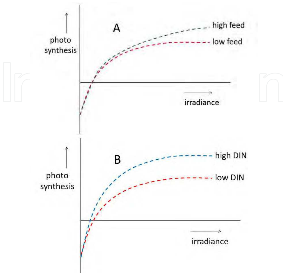
Fig. 10. Schematic representation of the findings of Houlbrèque et al. (2004) on the effects of feeding on photosynthesis in Stylophora pistillata (A) and the findings of Marubini & Davies (1996) on the effects of DIN enrichment on photosynthesis in Montastrea annularis and Porites porites (B).
