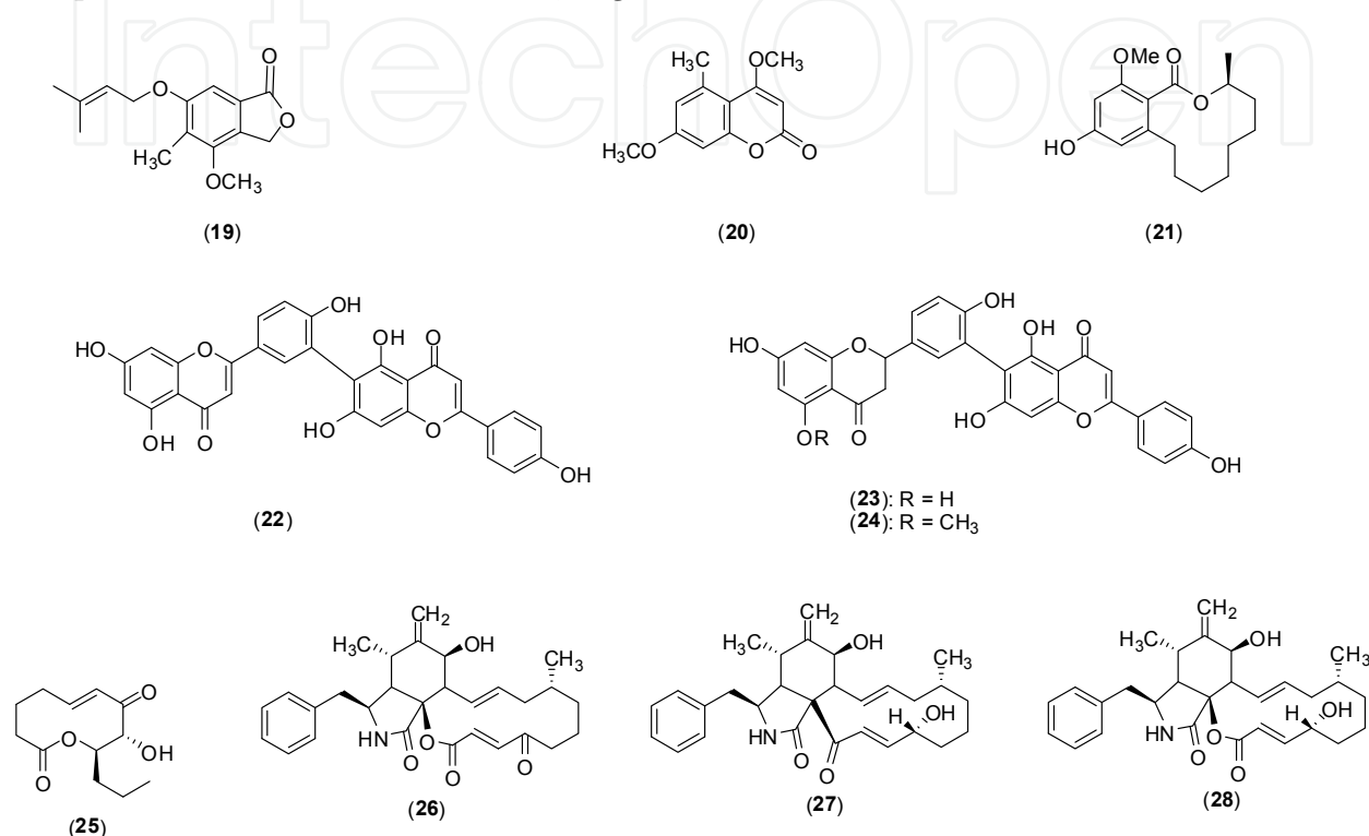
Fig. 6. Structures of compounds 19-28 mentioned in the text.
