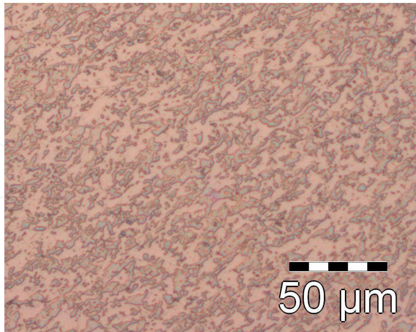
Fig. 1. CuCrZr microstructure.
