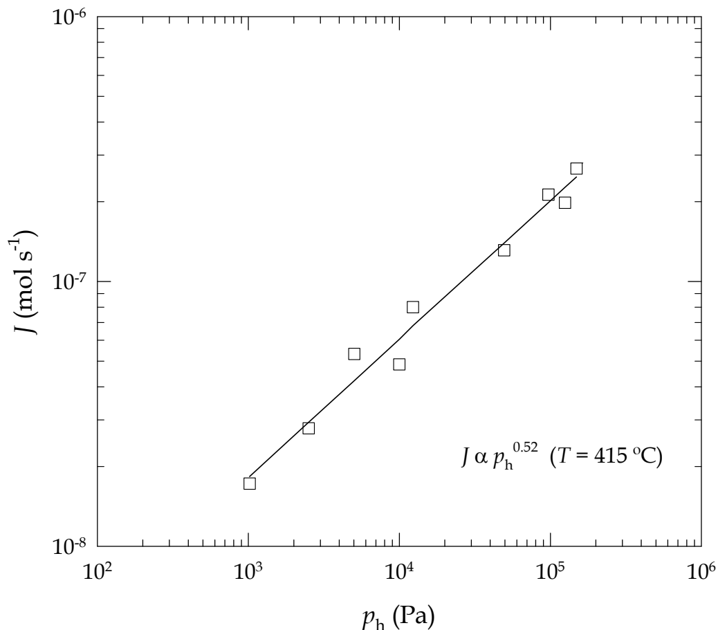
Fig. 6. Experimental hydrogen permeation steady-state flux in PH-CuCrZr alloy (ELBRODUR®) at 688 K and different driving pressures ranging from 10^3 to 1.5 \cdot 10^5 Pa.
