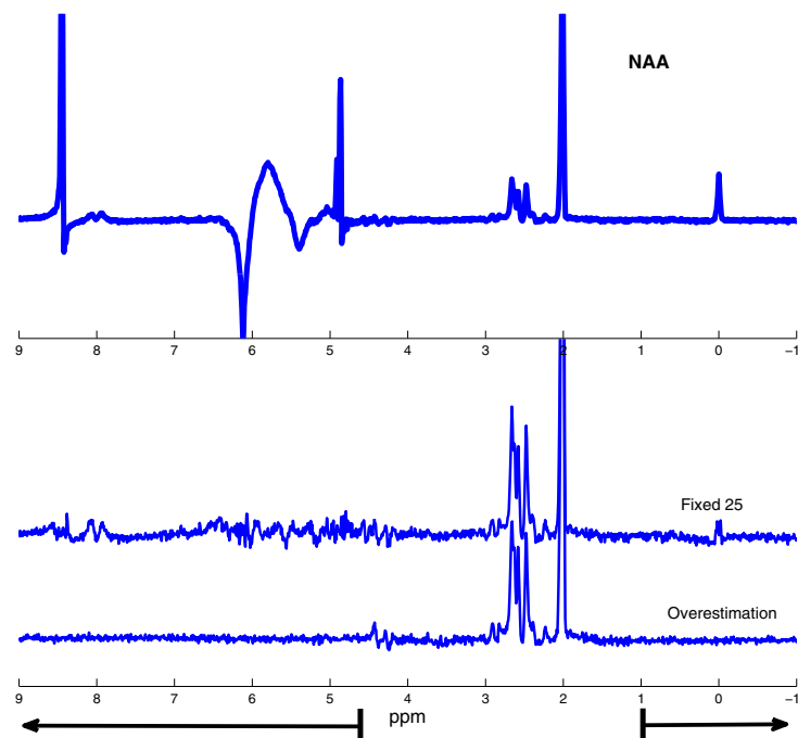
Fig. 4. Top: Real part of the spectrum of in vitro NAA measured at 1.5 T with acquisition parameters: Philips scanner, PRESS sequence, TR=6 s, TE=23 ms, SW=1 KHz, NDP=2048 points and 128 averages. Bottom: filtered signals using HLSVD-PRO with the model orders of K = 25 and overestimated as K = 309 . All modeled peaks in the frequency region outside the interval [1 ppm, 4.44 ppm] were suppressed. Residual resonances are visible for K = 25 in the water and reference peak regions, i.e. , 4.7 ppm, 0 ppm and 8.44 ppm.
