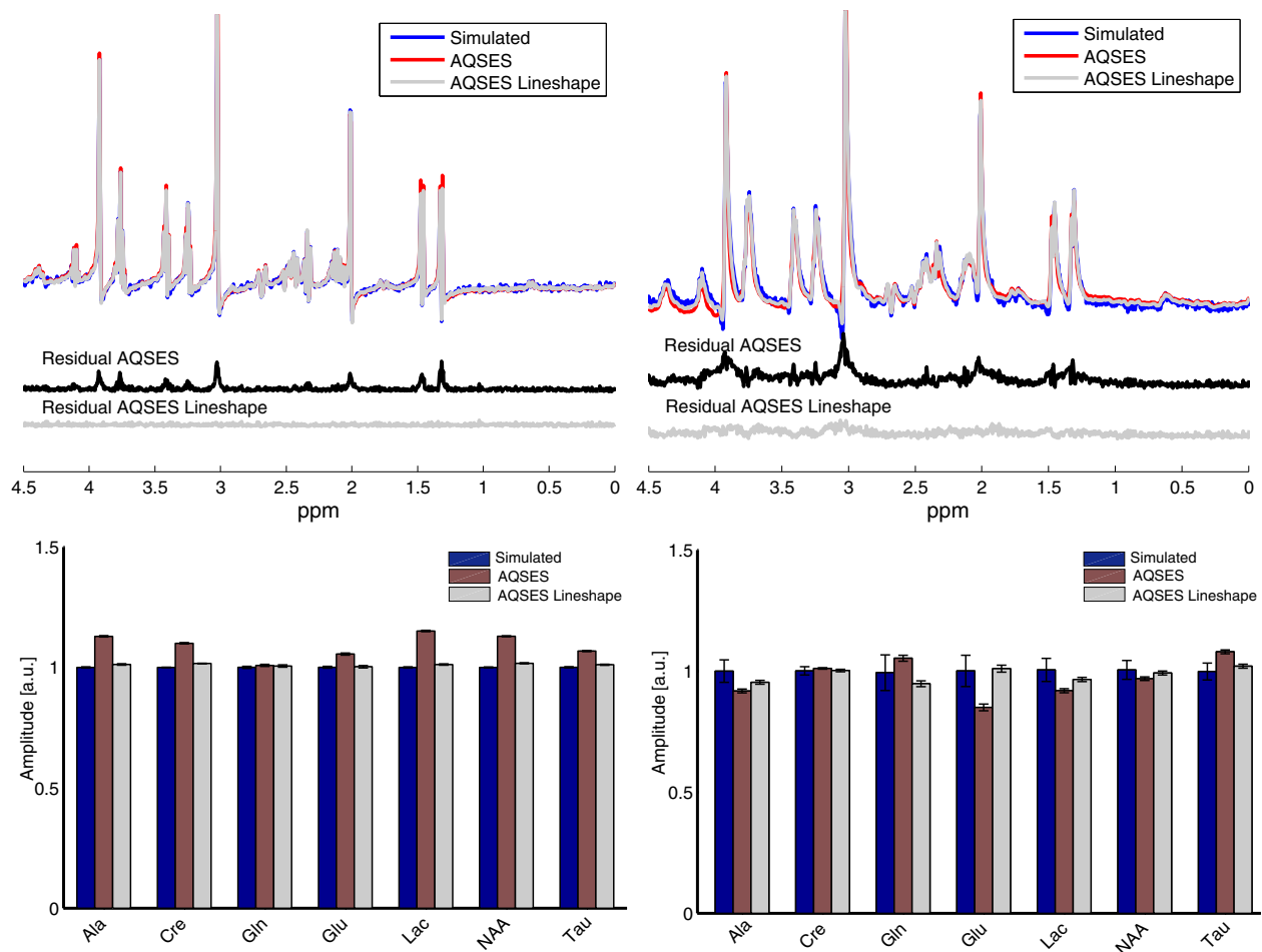
Fig. 8. Simulated MRS signals with lineshape distortions and the corresponding quantification results. These signals were obtained as the linear combination of 7 metabolites (Ala, Cr, Gln, Glu, Lac, NAA, and Tau) measured in vitro at 9.4 T with acquisition parameters: PRESS sequence, TR=8 s, TE=20 ms, SW=4 KHz and NDP=2048 points and 64 averages. Top left: small damping (to simulate in vitro signals). Top right: large damping (to simulate in vivo signals). The bottom plots represent the amplitude estimates for the corresponding simulated signals using AQSES and AQSES Lineshape.
