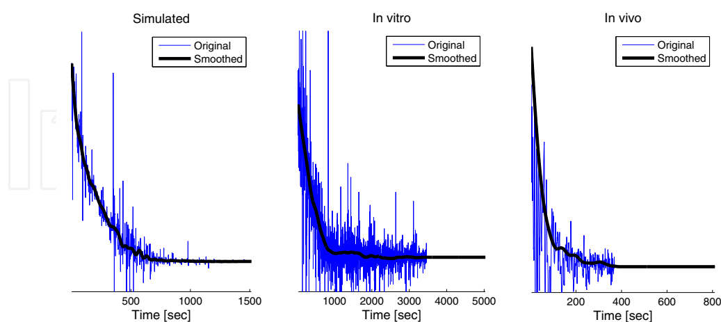
Fig. 7. Time domain signal of the resulting lineshape for simulated (left), in vitro (middle) and in vivo (right) signals. The signal labeled as 'Original' corresponds to the g(t) function calculated with the ratio formula in Eq.(3) and the smoothed signal is its final denoised version after convergence.
