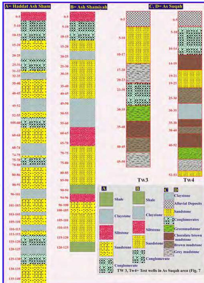
Fig. 10. Stratigraphic logs of the drilled test wells in Usfan basin (Modified from Sharaf, 2010a, b and 2011b).
