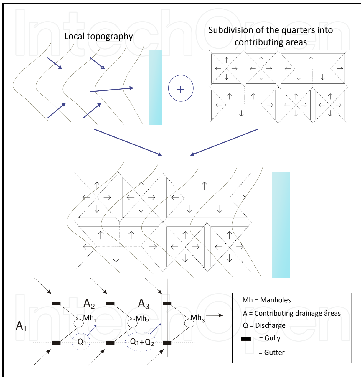
Fig. 2. Schematic urban drainage system classic design.
