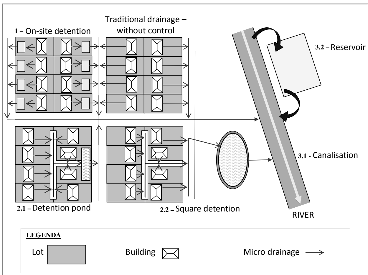
Fig. 3. Examples of flood control measures according to their working principle: 1. Distributed Measures; 2. Measures in the micro drainage; 3. Measures in the macro drainage (Rezende, 2010).
