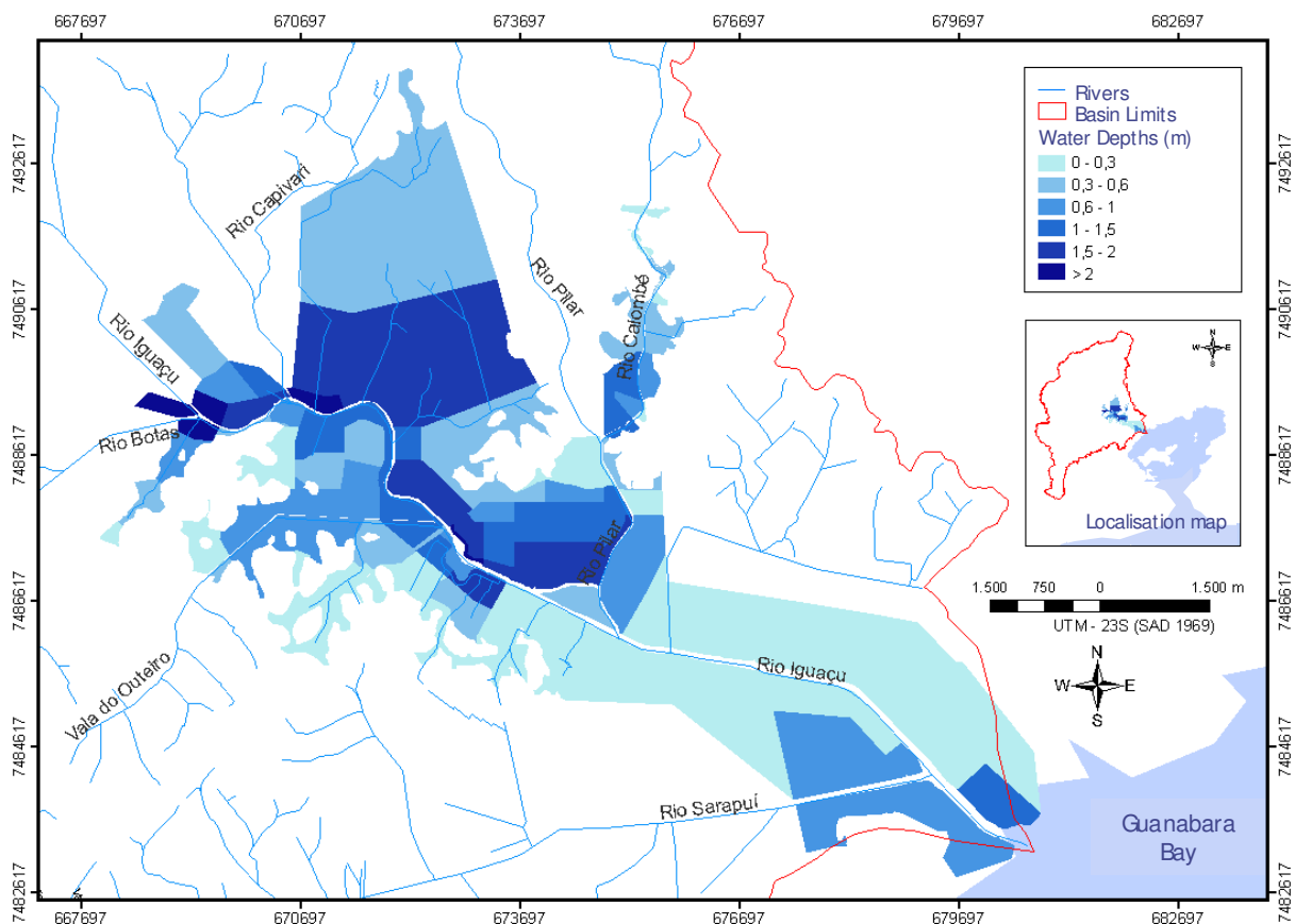
Fig. 7. Flood map of Iguaçu River Basin, for a design rainfall of 20 years of return period, calculated with a mathematical model aid.
