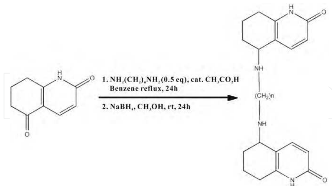
Fig. 2. Synthesis of bis(n)-hupyridones.
