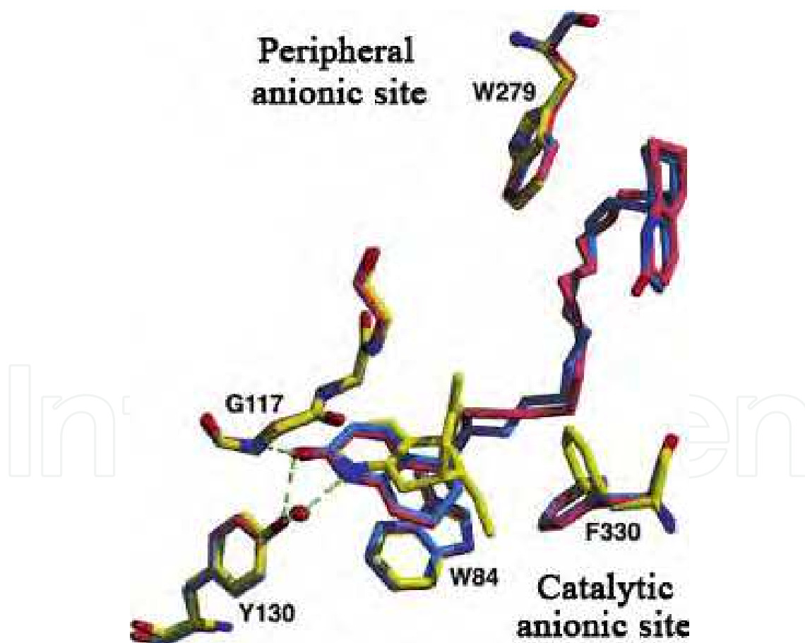
Fig. 3. Overlay of the refined structures of TcAChE /(-)-bis(10)-hupyridone (sky blue), TcAChE /(-)-bis(12)-hupyridone (pink), and TcAChE /(-)-huperzine A (yellow). Inhibitors and protein residues are rendered as sticks, and water molecules are shown as red spheres. The figure is modified from the reference (Wong et al., 2003).
