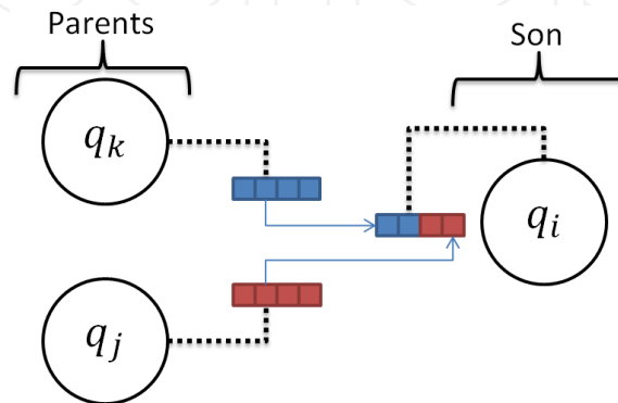
Fig. 13. Crossover between two solutions. Solutions of the states q_k and q_j are crossed in order to get state q_i
