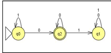
Fig. 5. Automata state diagram for the example 1.
