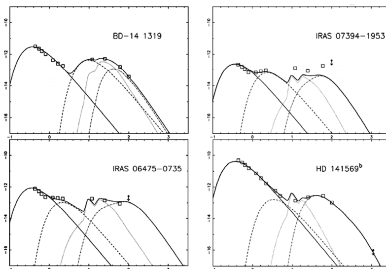
Fig. 4. GA SEDs obtained the stars BD-14 1319, IRAS 07394-1953, IRAS 06475-0735 and HD 141569. The plots are given as \log[\lambda F_\lambda(\text{Wm}^{-2})] versus \log[\lambda(\mu\text{m})] (Hetem & Gregorio-Hetem 2007).
