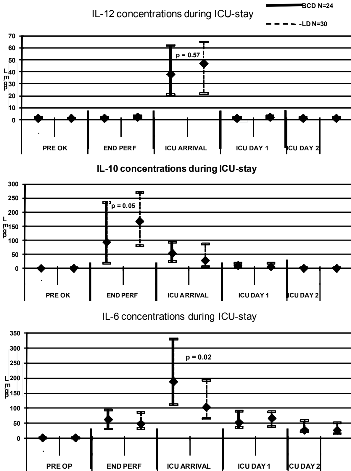
Fig. 1. Pre-operative (PRE OP), at end of perfusion (END PERF), at arrival at ICU (ICU ARRIVAL) and at days 1 and 2 (ICU DAY 1 and 2) the concentrations of cytokines (IL-6, IL-10 and IL-12) (Bilgin et al., 2010).
