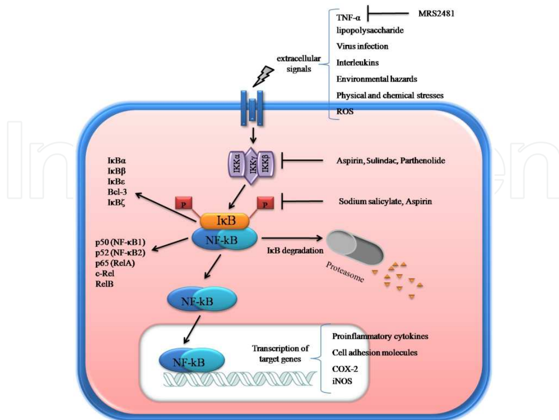
Fig. 1. Schematic representation of NF- \kappa B activation in inflammatory disease. A variety of upstream extracellular signals activate the IKK complexes, which are comprised of 3 subunits: IKK \alpha , IKK \beta , and IKK \gamma . Phosphorylation of I \kappa B by the IKK complex in the N-terminal regulatory domain at two critical serine residues results in the ubiquitination and subsequent degradation of I \kappa B by proteasome. Free NF- \kappa B dimers translocate into the nucleus, where they bind to specific promoters and affect gene transcription of such molecules as proinflammatory cytokines, cell adhesion molecules, COX-2, and iNOS. Some drugs and agents are able to suppress NF- \kappa B activation via different pathways. Aspirin and sodium salicylate block I \kappa B phosphorylation and degradation. Sulindac, Parthenolide, Aspirin inhibit activation of the NF- \kappa B pathway by suppressing IKK activity and MRS2481 inhibit TNF- \alpha .
