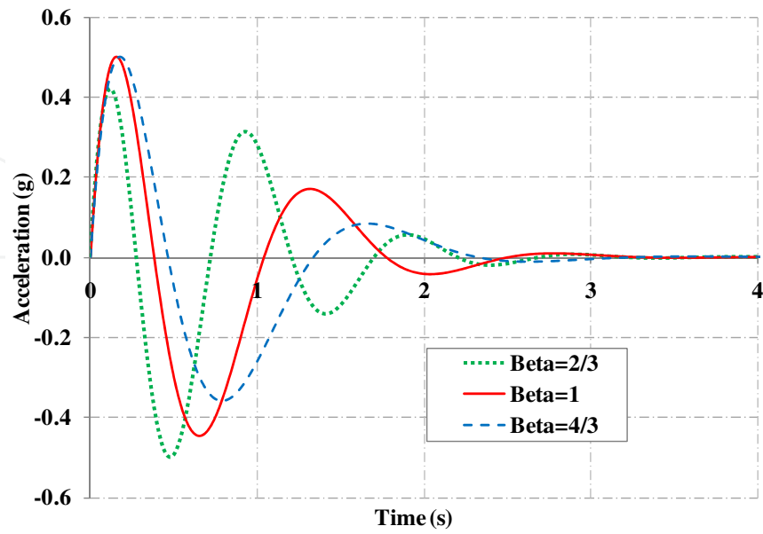
Fig. 7. Time-history plots of acceleration for \beta = 2/3, 1, 4/3 .
