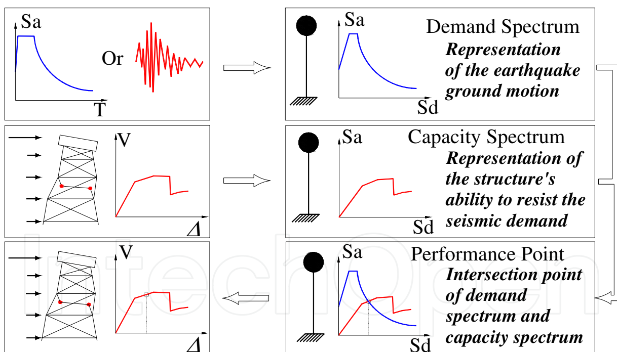
Fig. 3. Capacity-spectrum method.
