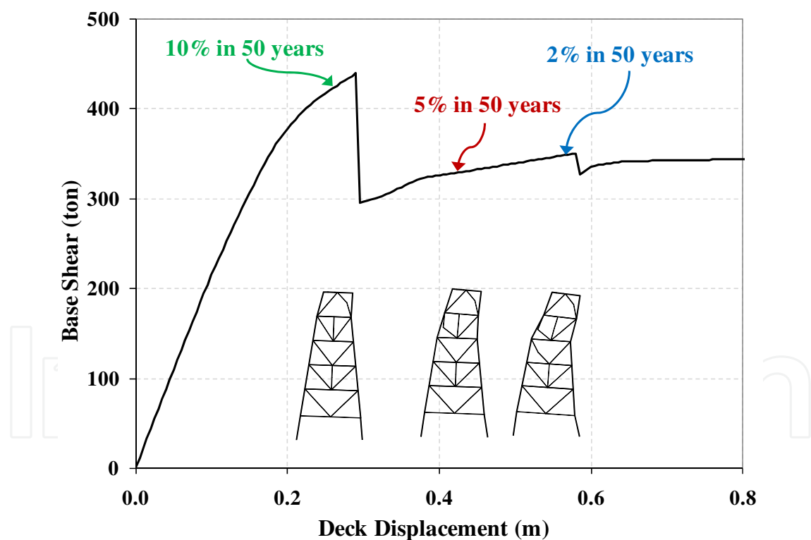
Fig. 6. Performance of the jacket for various levels of hazard.
