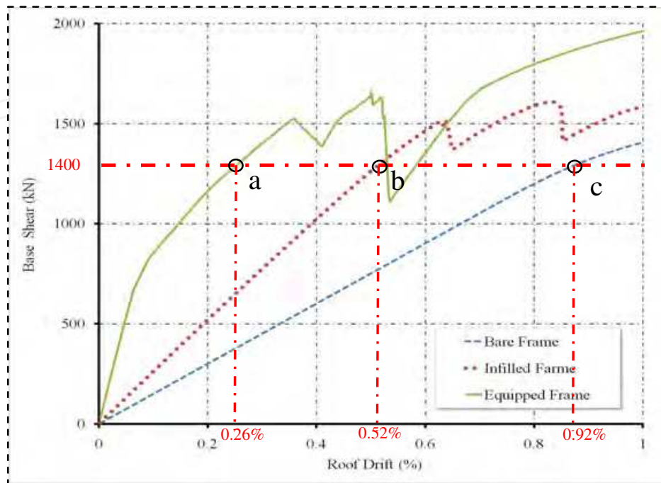
Fig. 14. Pushover curves
