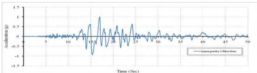
Fig. 16. Acceleration Time History of Loma Perita Earthquake
