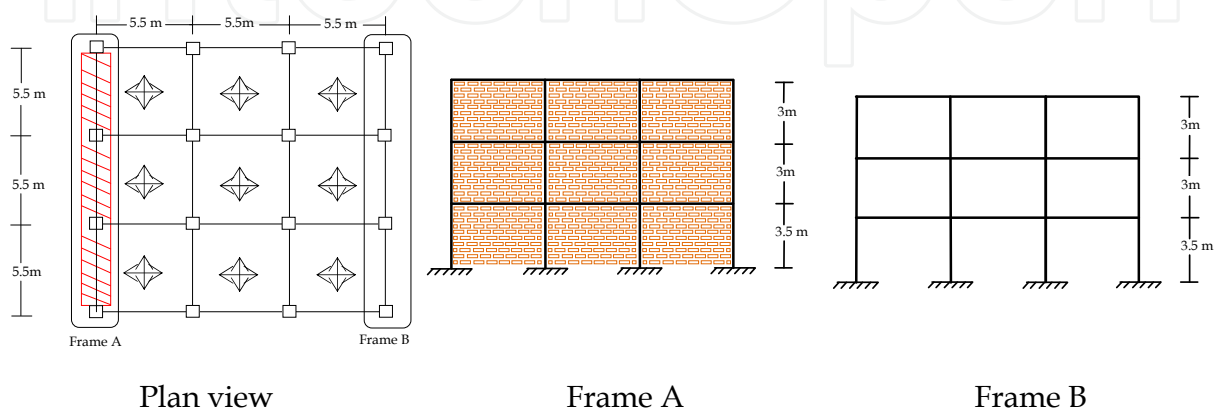
Fig. 13. Building elevation
