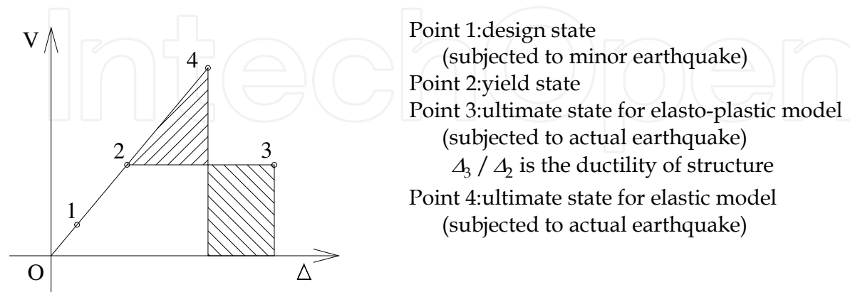
Fig. 11. Idealized curve of storey shear force vs. storey drift
