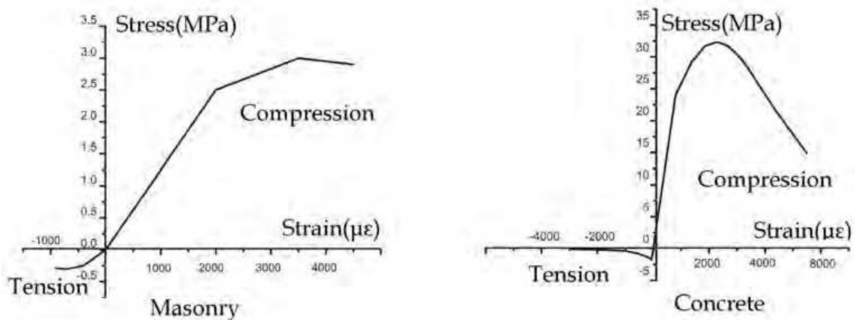
Fig. 16. Constitutive model for masonry and concrete
