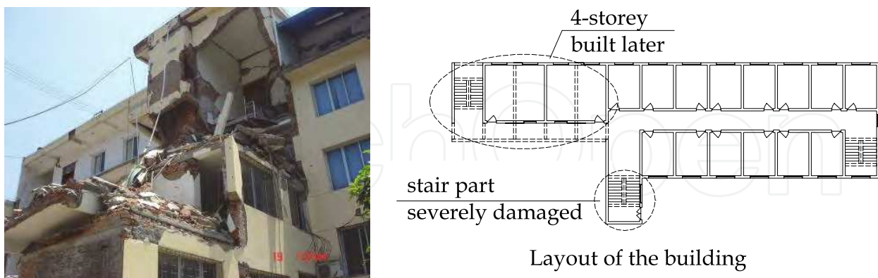
Fig. 3. Partial collapse of stair part
