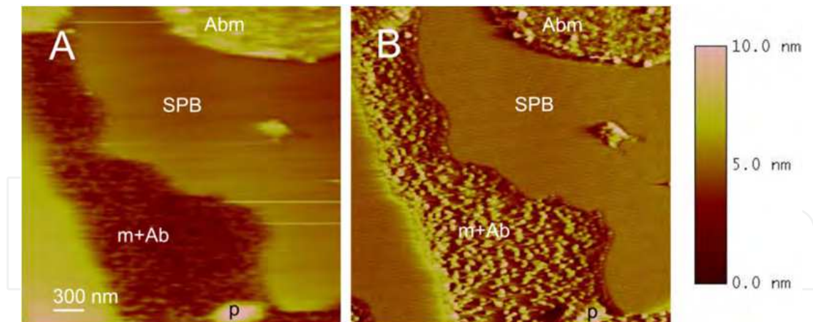
Fig. 9. AFM height and deflection images of IgG adsorption (10 g/l in HBS containing 1.5 mM of calcium) to mica patches of discontinuous SPB, measured in the contact mode fluid cell. (A) On the image, three surfaces can be observed: loose antibody layer on mica (Abm) that can be measured around 5 nm above SPB; the SPB layer (SPB), about 4 nm above mica; and mica with some antibodies that only started to adsorb or accumulate (m+Ab). One can deduce that assemblies on m+Ab, representing IgG, started randomly interconnect with each other to form the loose antibody patch on mica (p). On the Abm, the antibody patch is already formed. No binding of antibodies to the SPB was measured. (B) The deflection image of the same surface as in image A. All three surfaces can be more clearly observed. Globular assemblies can be deduced.
