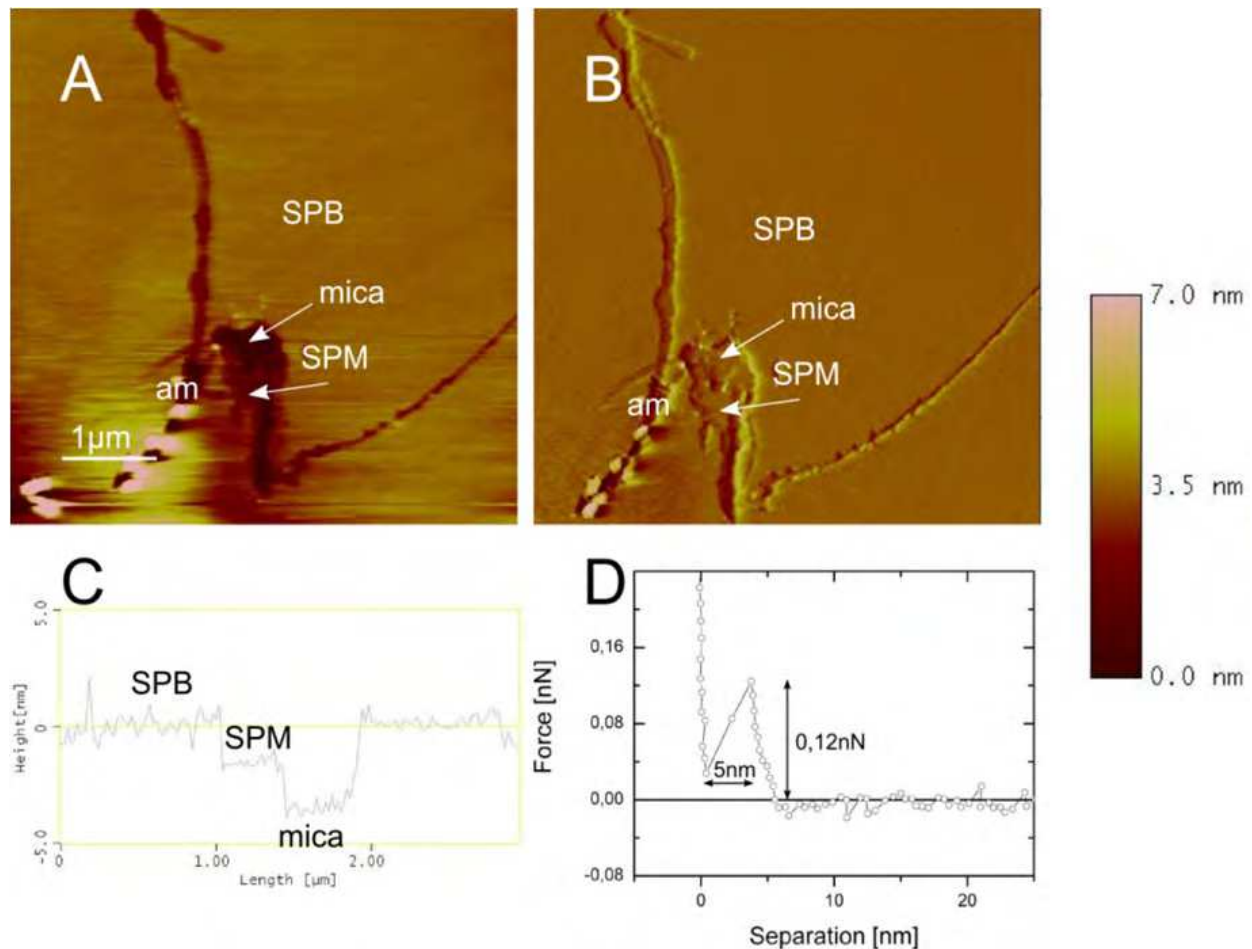
Fig. 3. AFM height and deflection images, height cross section and force measurement of SPB, disrupted with the AFM tip and measured in the contact mode AFM fluid cell. As a buffer above SPB, HBS with 2 mmol/l of calcium was used. This figure presents evidence that the phospholipid vesicles form phospholipid bilayer and not monolayer on mica. (A) AFM height image, where three layers: mica, first phospholipid monolayer (SPM) and second monolayer, which together form the SPB, are measured. Some accumulated material (am) can also be deduced. (B) AFM deflection image of the same surface as in image A, where all three layers are more clearly visible. (C) Height cross section of image A, indicating first phospholipid monolayer is 2 nm higher and the phospholipid bilayer is 4 nm higher than mica. (D) Force measurement showing that the tip is penetrating through SPB about 5 nm thick, with the required force for penetration of 0.12 nN.
