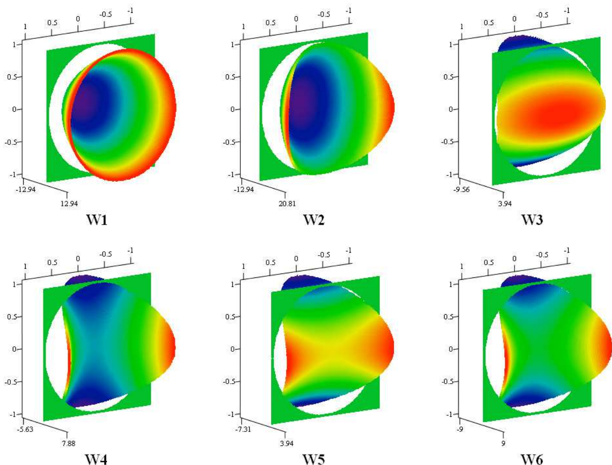
Fig. 1. Three-dimensional 2 nd order wave front maps
