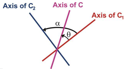
Fig. 10. Composition of two obliquely crossed cylinders with cylindrical powers of C_1 and C_2 (C: resultant cylinder).
