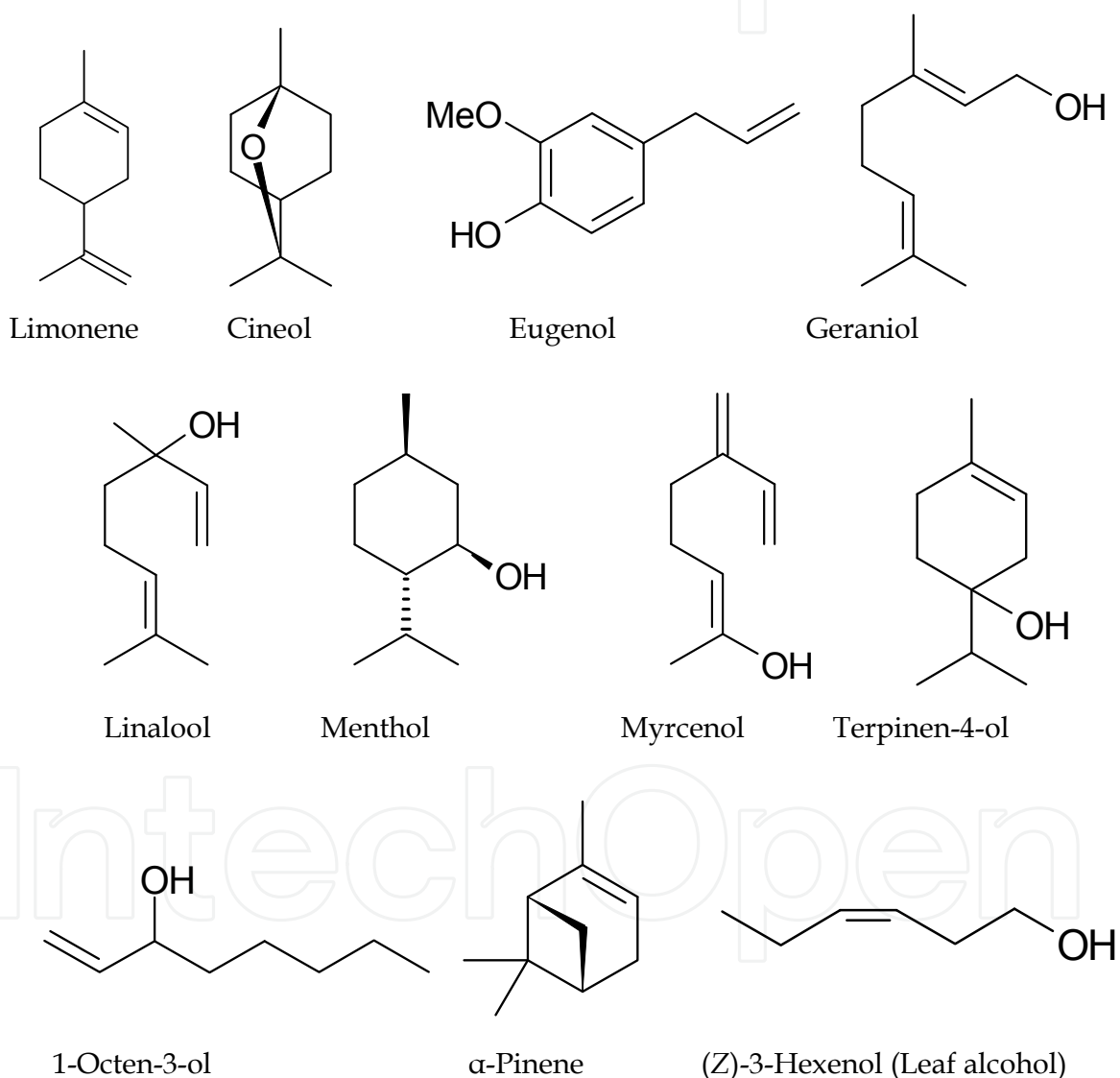
Fig. 1. Chemical structure of several popular fragrant compounds.
