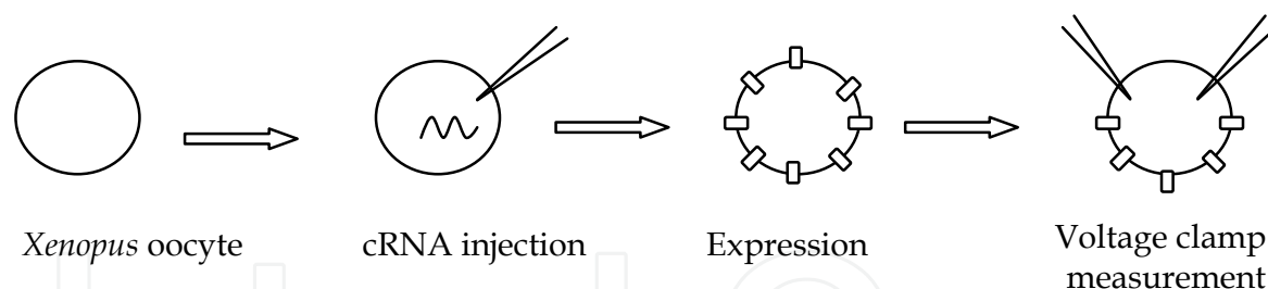
Fig. 5. The experimental procedures using the Xenopus oocyte expression system and electrophysiological measurements to examine the effects of fragrant compounds on the response of GABA A receptors.
