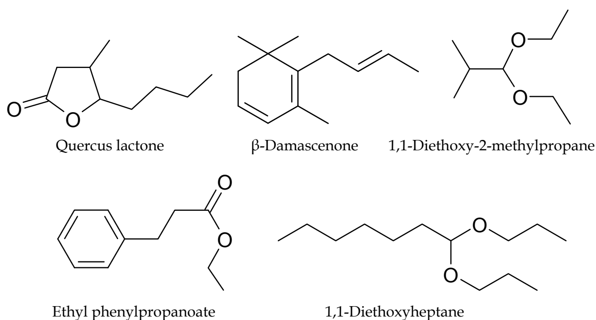
Fig. 2. Some fragrant compounds in whiskey (or whisky).
