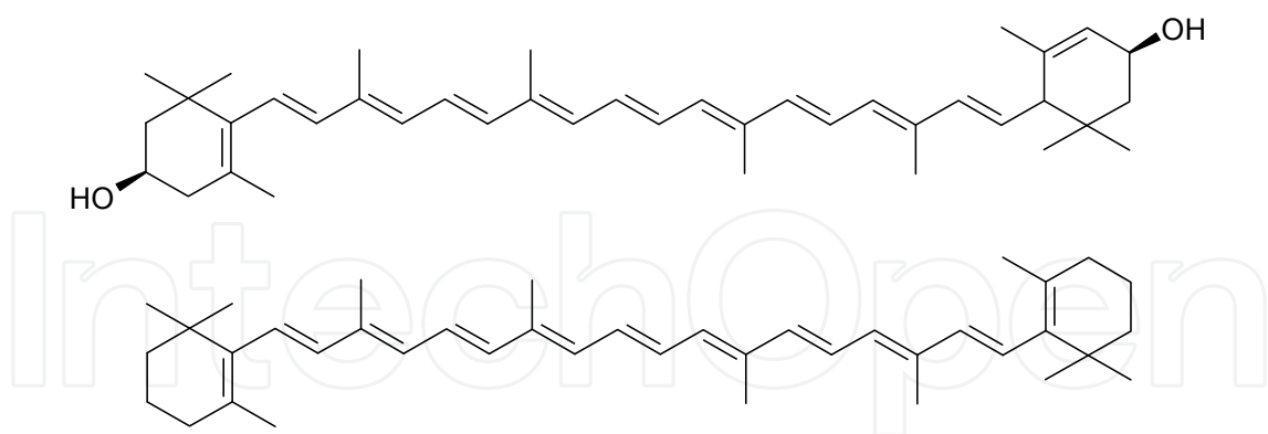
Fig. 2. Chemical structures of the carotenoids lutein (above) and \beta -carotene (below).
