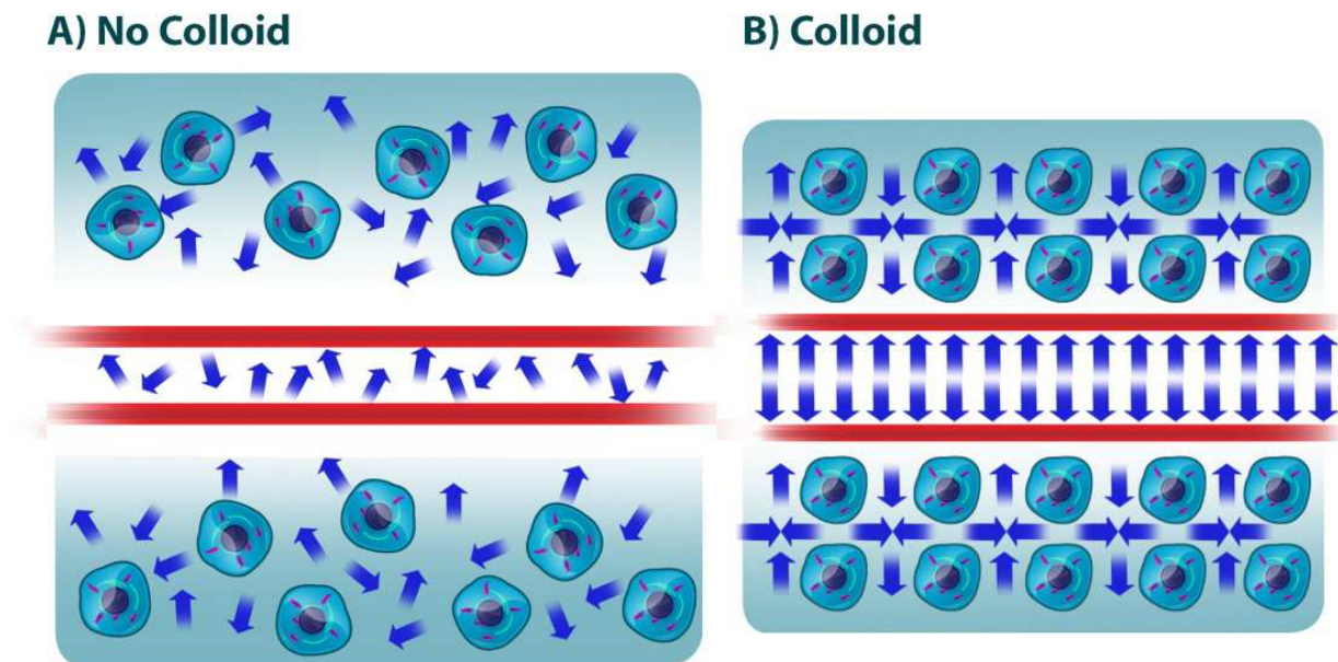
Fig. 5. Osmotic colloidal pressure.
