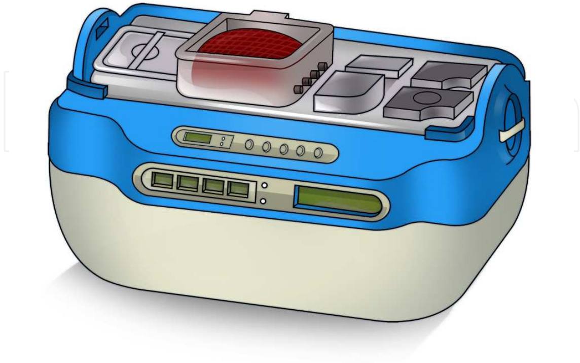
Fig. 2. Hypothermic perfusion machine: Life Port Kidney Transporter® from Organ Recovery Systems®.
