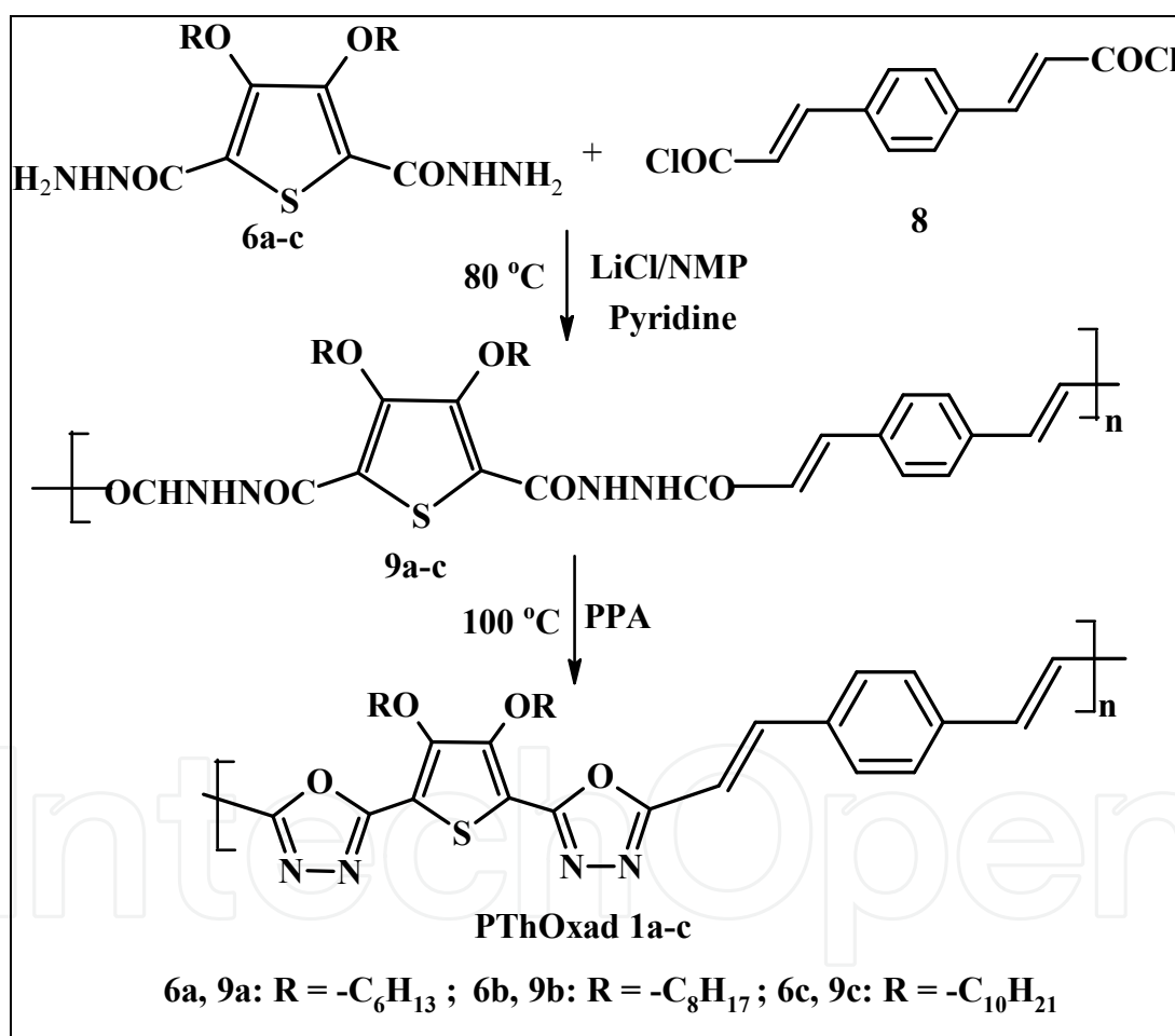
Scheme 3. Synthesis of polymers, PThOxad 1a-c.
