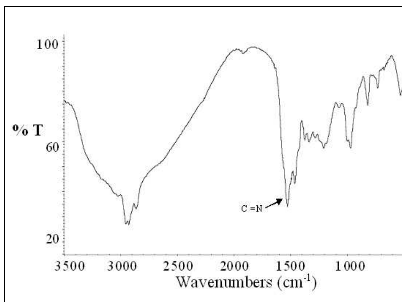
Fig. 4. FT-IR spectrum of polyoxadiazole, PThOxad 1c.
