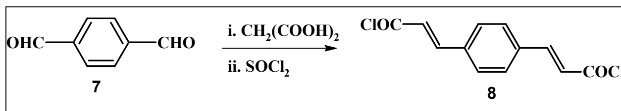
Scheme 2. Synthesis of 3,3'-(1,4-phenylene)bis[2-propenoyl chloride] (8)
