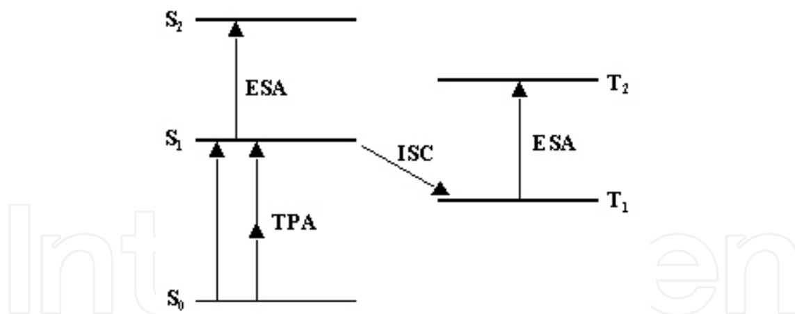
Fig. 14. Energy level diagram showing both two-photon absorption and excited state absorption.
