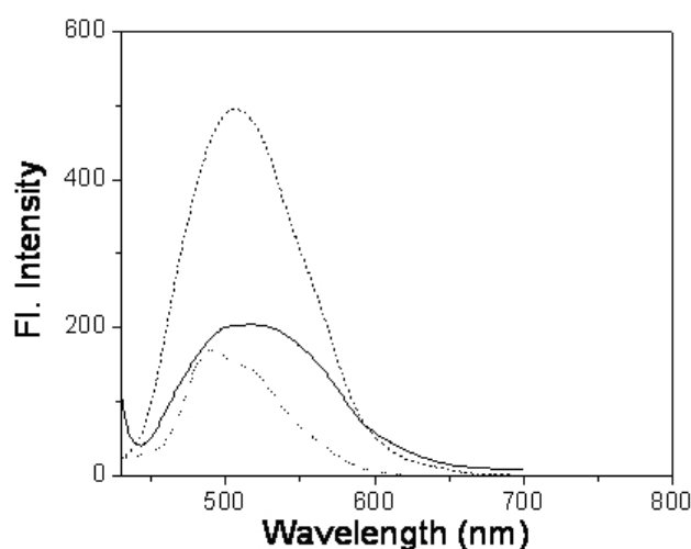
Fig. 12. Fluorescence emission spectra of the polymer solution in chloroform (---), polymer film (—) and nanocomposite film (...).
