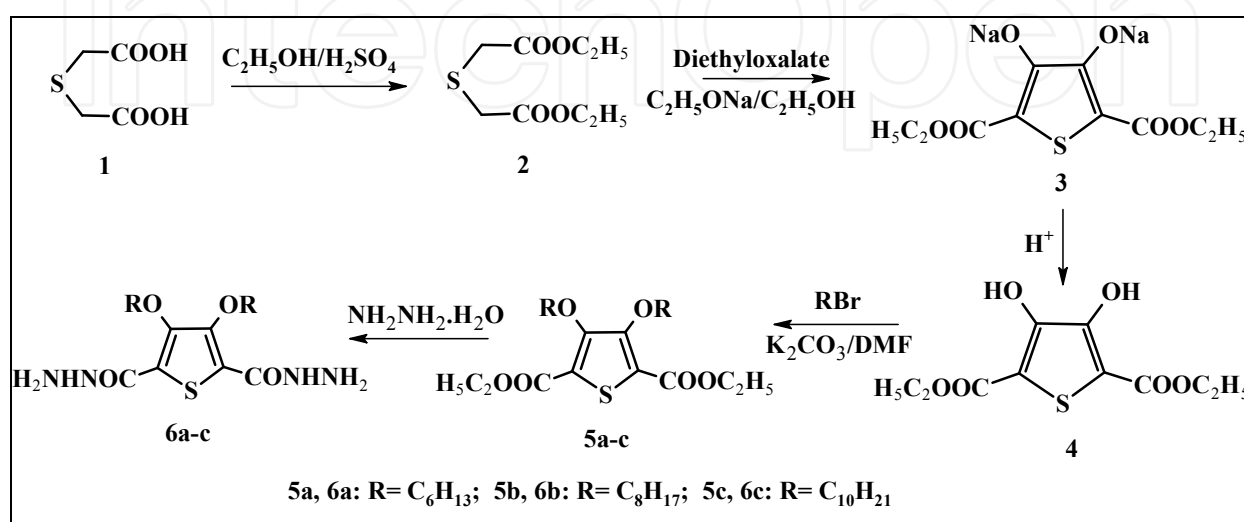
Scheme 1. Synthesis of 3,4-dialkoxythiophene-2,5-carbonyldihydrazides (6a-c).
