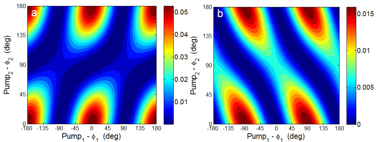
Fig. 3. Noncollinear second harmonic signal theoretically calculated as a function of the polarization state of the first pump beam ( \phi_1 ) and the second pump beam ( \phi_2 ). Sample rotation angle was fixed to \alpha=35^\circ . The polarization state of the analyzer is set to (a) \hat{p} i.e. \phi=0^\circ and (b) \hat{s} , i.e. \phi=90^\circ .
