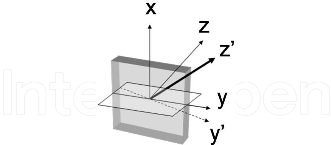
Fig. 8. Sketch of the film orientation. z and z' represents the optical axis orientation before and after rotation about the x -axis, respectively.
