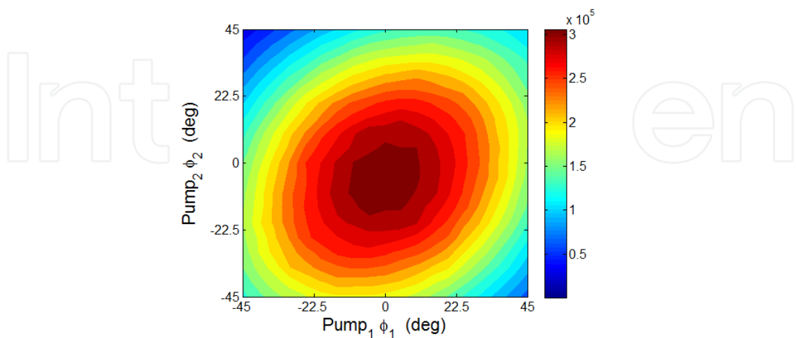
Fig. 11. Detail of the noncollinear second harmonic signal experimentally measured as a function of the polarization state of both pump beams, i.e. \phi_1 and \phi_2 . Sample rotation angle was \alpha = -40^\circ . The polarization state of the analyzer is set to \hat{p} i.e. \phi = 0^\circ .
