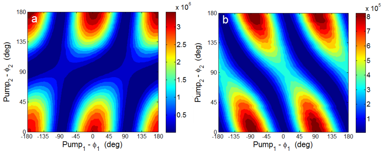
Fig. 2. Noncollinear second harmonic signal experimentally measured as a function of the polarization state of the first pump beam ( \phi_1 ) and the second pump beam ( \phi_2 ). Sample rotation angle was fixed to \alpha=35^\circ . The polarization state of the analyzer is set to (a) \hat{p} i.e. \phi=0^\circ and (b) \hat{s} , i.e. \phi=90^\circ .
