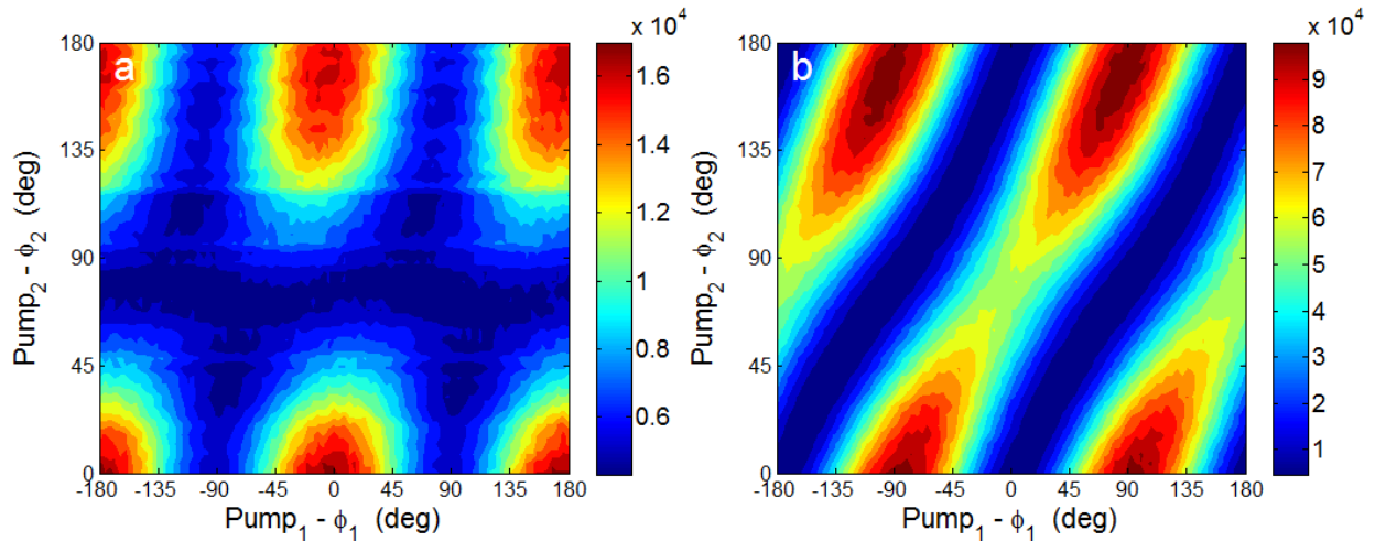
Fig. 4. Noncollinear second harmonic signal experimentally measured as a function of the polarization state of the first pump beam ( \phi_1 ) and the second pump beam ( \phi_2 ). Sample rotation angle was fixed to \alpha=1^\circ . The polarization state of the analyzer is set to (a) \hat{p} i.e. \phi=0^\circ and (b) \hat{s} , i.e. \phi=90^\circ .
