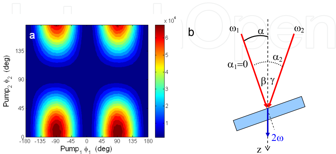
Fig. 6. (a) Noncollinear SH signal measured as a function of the polarization state of the first pump beam ( \phi_1 ) and the second pump beam ( \phi_2 ). The polarization state of the analyzer is set to \hat{s} , i.e. \phi=90^\circ . (b) Sketch of the experimental configuration: sample rotation angle was fixed to \alpha=9^\circ .
