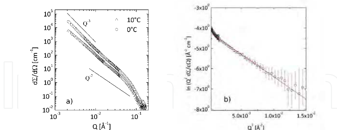
Fig. 22. SANS patterns under wax contrast from a 1% tetra-block and 1% C_{30} +1% C_{36} solution in decane (a) and the Guinier presentation of the large Q data at 0^{\circ}\text{C} , delivering in a direct approach the thickness and the “forward scattering” of the wax lamellae (b).
