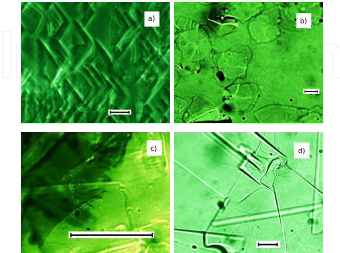
Fig. 8. Micrographs from decane solutions of mixed 1% C_{36} /1% C_{30} at 0°C (a), 0.5% C_{24} at -20°C (b), 1% C_{36} at 20°C (c) and 4% C_{24} at -10°C (d); scale bars 30 \mu m.
