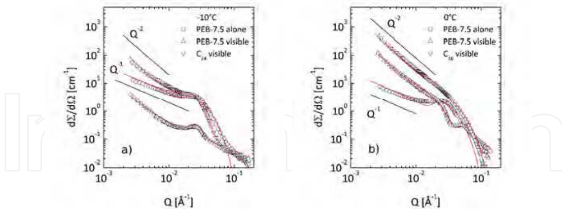
Fig. 14. Examples of wax and polymer SANS profiles (triangles) from PEB- n /wax mixed solutions in decane (Radulescu et al., 2004) for 0.6%PEB-7.5/1% C_{24} at -10^{\circ}\text{C} (a) and 0.6%PEB-7.5/0.5% C_{36} at 0^{\circ}\text{C} (b); the polymer self-assembling SANS patterns (circles) are shown in parallel in order to emphasize the structural changes induced by the addition of wax; the curves represent model description of the data (see text).
