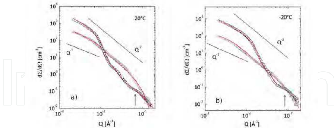
Fig. 18. Examples of SANS patterns measured from mixed 1%tetra-block/1% C_{36} (a) and 1%tri-block/1% C_{24} (b) decane solutions for the polymer (circles) and wax (triangles) visible; the red curves denote the model interpretation of data while the arrows indicate the high- Q scattering detail characteristic for polymer blobs.
