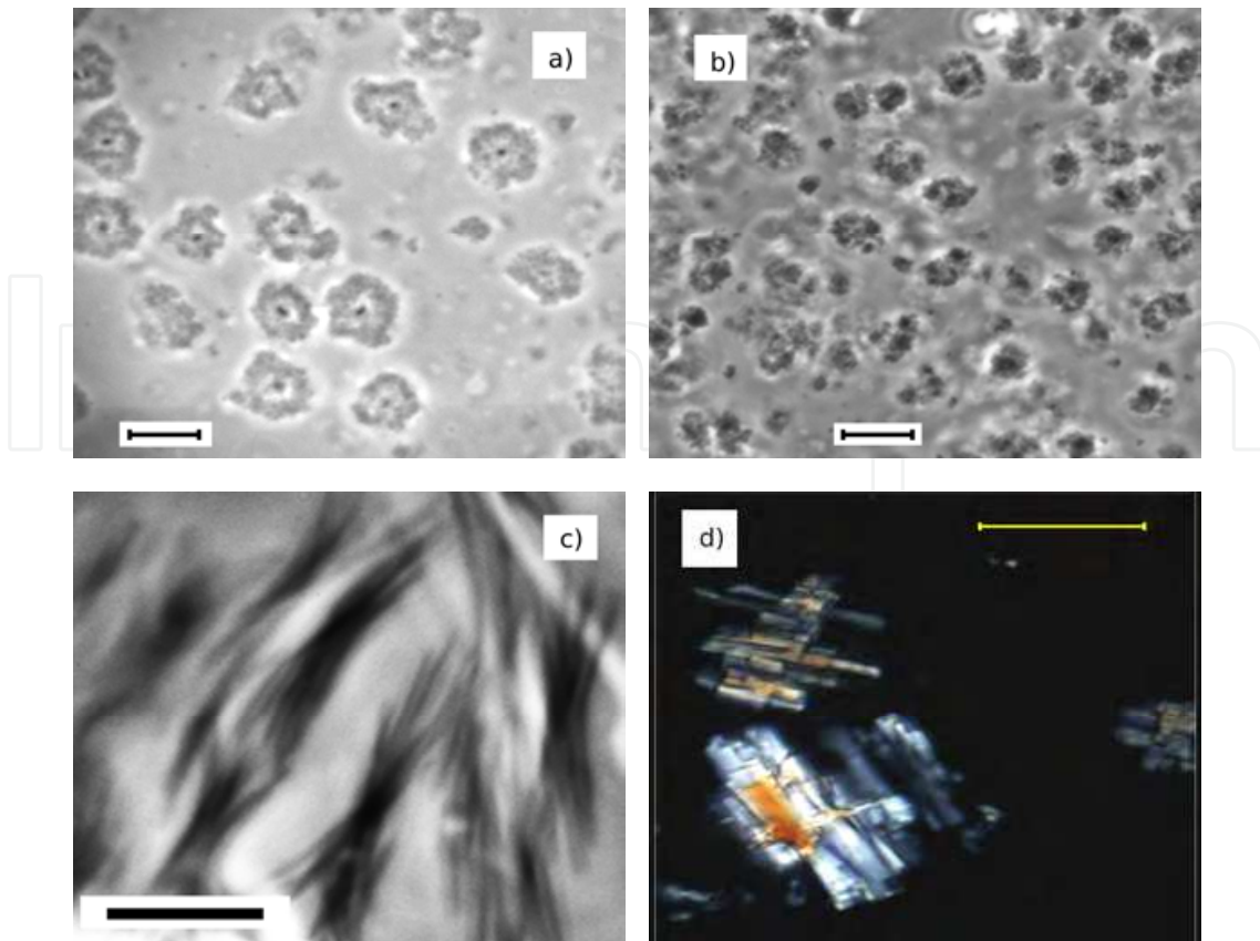
Fig. 17. Aggregates formed at 0°C in decane solution of 1% tetra-block copolymer with no wax (a), 1% C 36 (b) and 4% C 36 (c,d) added as revealed by bright field (a-c) and crossed polarizers (d) microscopy (Radulescu et al., 2011); the scale bar: 10μm (a-c), 20μm (d).
