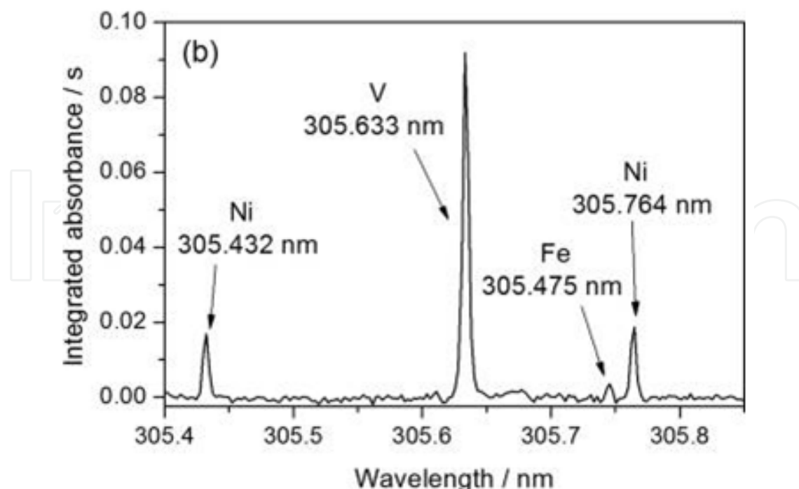
Fig. 1. Absorbance spectrum for the OB-2 crude oil sample emulsion in the vicinity of the vanadium secondary line at 305.633nm, with a pyrolysis temperature of 1000 °C, Wavelength resolved integrated absorbance spectrum (Quadros et al. 2010) with permission.
