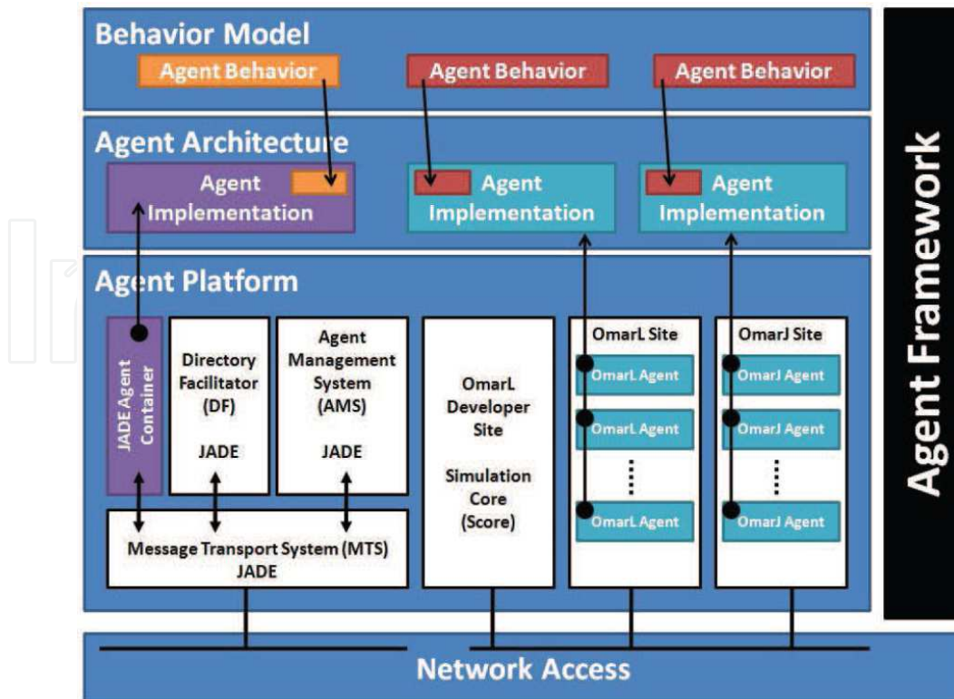
Fig. 2. Description of Agent Framework.
