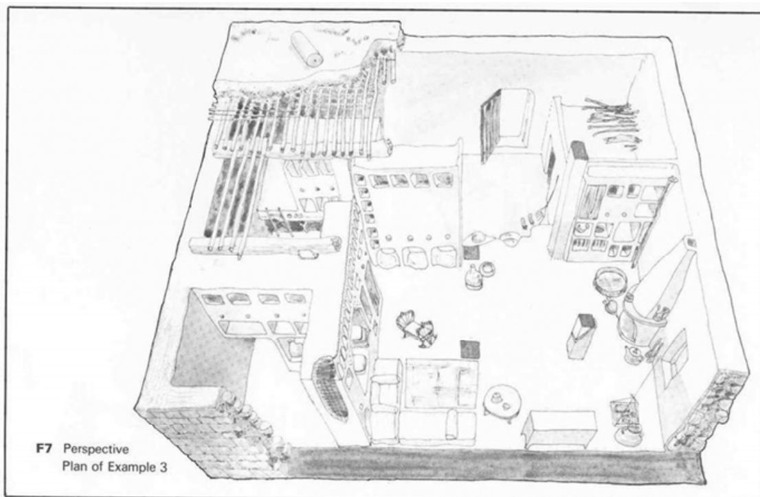
Fig. 9. Three dimensional construction of the Bait Al Fallah , folkloric museum of Ebel-es-Saqi as surveyed by Frederic Ragette (1980)
