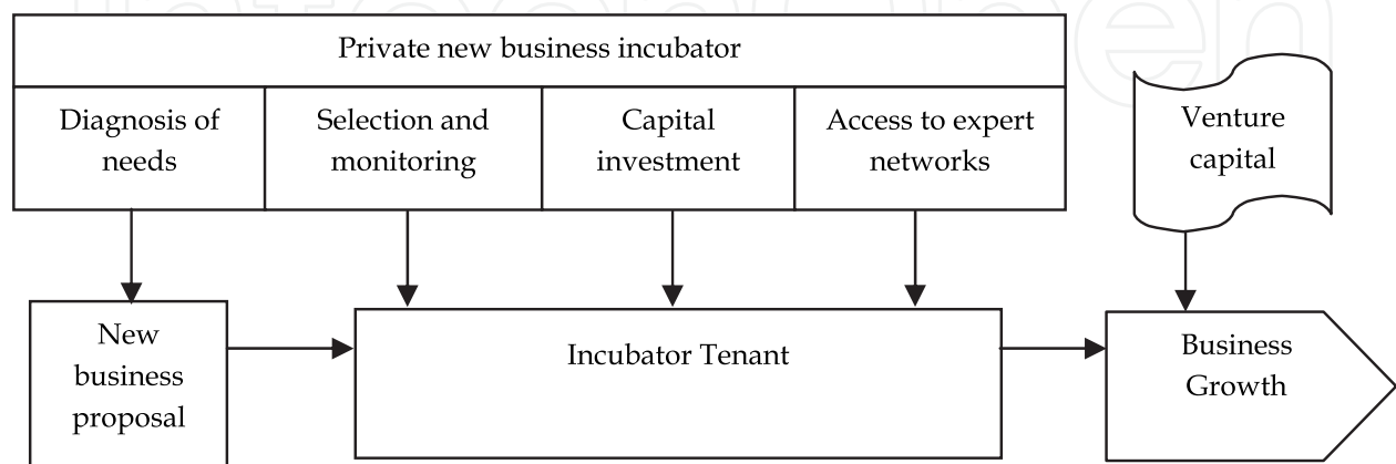
Fig. 2. Campbell, Kendrick & Samuelson's (1985) incubation model
