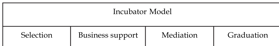
Fig. 4. Bergek & Norrman's (2008) incubation model
