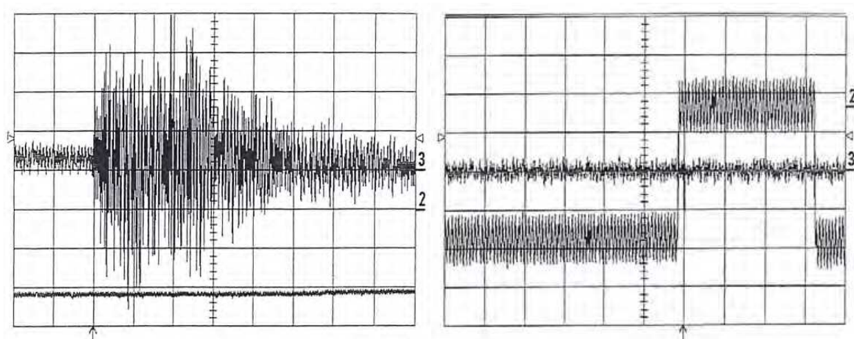
Fig. 12. Sporadic AE signal from the TWT-A in CW operation (left frame) and periodic AE signal on the sixth vertical division (compressed) from pulsing the TWT-A (right frame).
