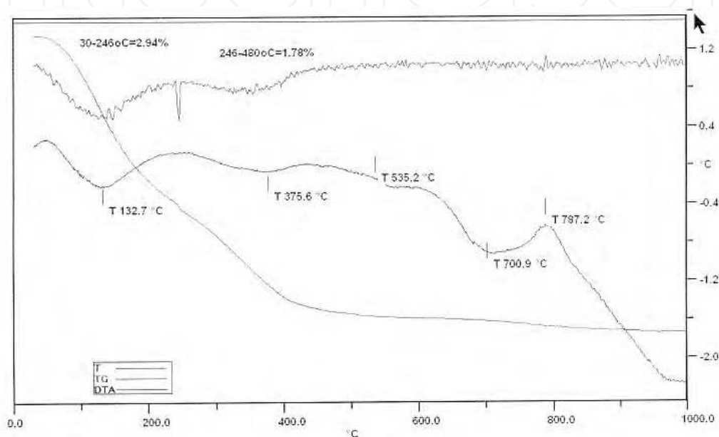
Fig. 7. DTA and DTG of glass FB2 system.
