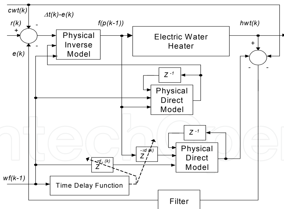
Fig. 8. SPC constituent blocks.
