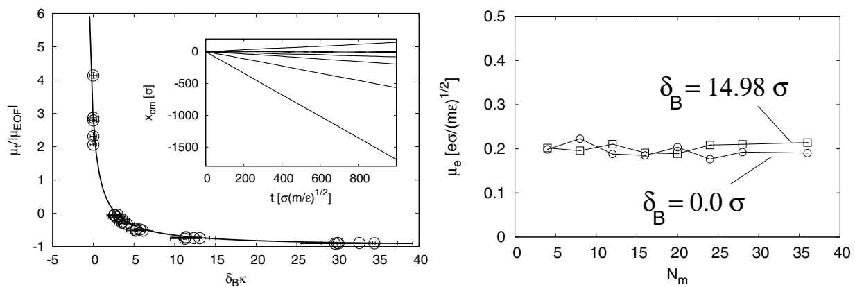
Fig. 3. Left side: Ratio \mu_t/|\mu_{EOF}| plotted against \delta_B \kappa_s for chains of length N_m = 20 and several slip lengths and salt concentrations. The black line is the theoretical prediction of Eqn. (46). The ratio \mu_e/\mu_{EOF}^0 has been fitted to -3.778 \pm 0.128 . Negative values of \mu_t/|\mu_{EOF}| indicate negative total mobilities of the polyelectrolyte. Inset: Total displacement of the polyelectrolyte's center of mass for different boundary conditions and a salt concentration of \rho_s = 0.05625\sigma^{-3} , in units of the ion diameter \sigma . The total mobility becomes negative for |\mu_e| \ll |\mu_{EOF}| . The lines correspond from top to bottom to the slip lengths \delta_B \approx (0.00, 1.292, 1.765, 2.626, 5.664, 14.98)\sigma . Thus larger slip lengths indirectly enhance the total mobility of the polyelectrolyte. Right side: Bare electrophoretic mobility for different monomer lengths N_m in confined geometry in the presence of salt for two slip lengths.
