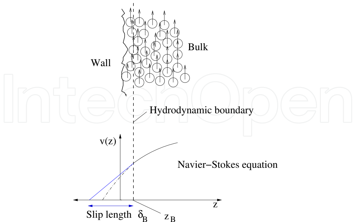
Fig. 1. Top: Coarse-grained schematic illustration of fluid flow in close vicinity to the boundaries. The hydrodynamic boundary is not identical to the fluid-solid interface due to atomistic roughness. Bottom: Flow profile in the direction normal to the hydrodynamic boundary. In close vicinity to the boundary, the Navier-Stokes equations are not valid. An extrapolation of the flow profile determines the slip length.
