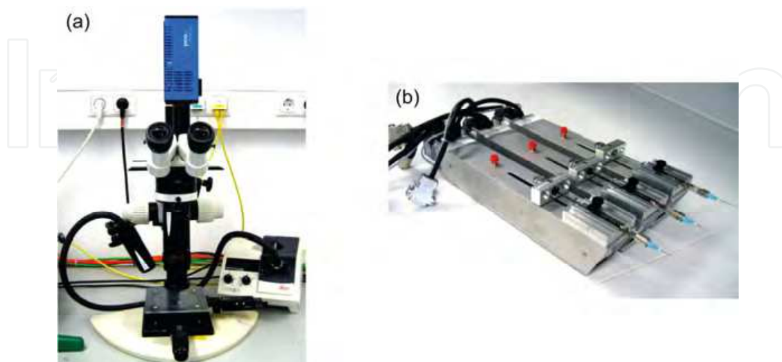
Fig. 3. a) Leica macroscope Z16 APO with a Leica L5 FL light source and camera. b) Custom made syringe pumps with glass syringes (Hamilton).
