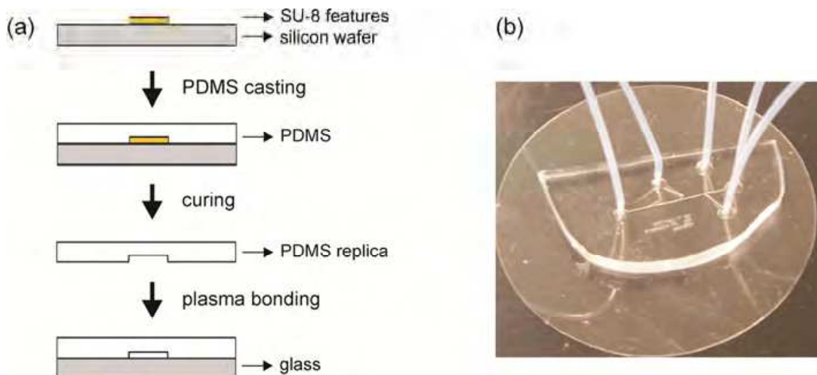
Fig. 2. (a) Schematic of PDMS Device Fabrication. (b) Ready to use PDMS device with tubes connected; the diameter of the cover glass slide: 5 cm.
