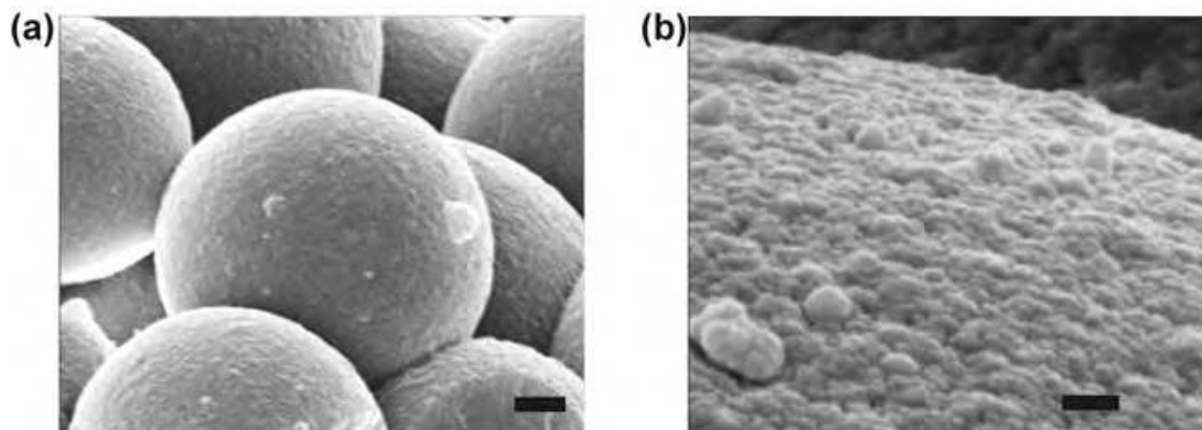
Fig. 10. Scanning electron micrographs of silica spheres after calcinations. (a) Scale bar: 1 \mu\text{m} . (b) Close up of the surface structure. Scale bar: 50 nm.
