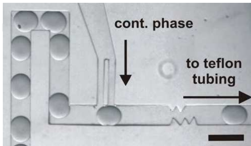
Fig. 8. Optical micrograph showing the end of the mixing line. The flow is from left to right. Right after the mixing line additional continuous oil phase is injected via the side channel to increasing the distance between the merged droplets before they enter the Teflon tubing. Scale bar: 200 \mu\text{m} .
