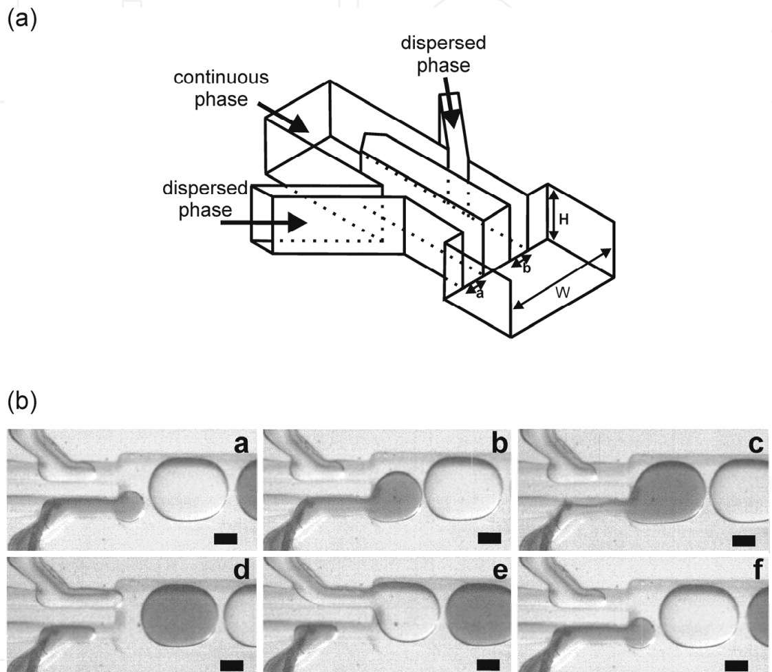
Fig. 4. (a) Schematic of the double step-emulsification device. The typical device dimensions were a = b = 35 \mu\text{m} , H = 120 \mu\text{m} and W = 160 \mu\text{m} . (b) Time series of optical images showing the droplet formation using a double step-emulsification device. For clarity, the aqueous phase injected from bottom is dyed with Nile blue. Scale bar: 50 \mu\text{m} .
