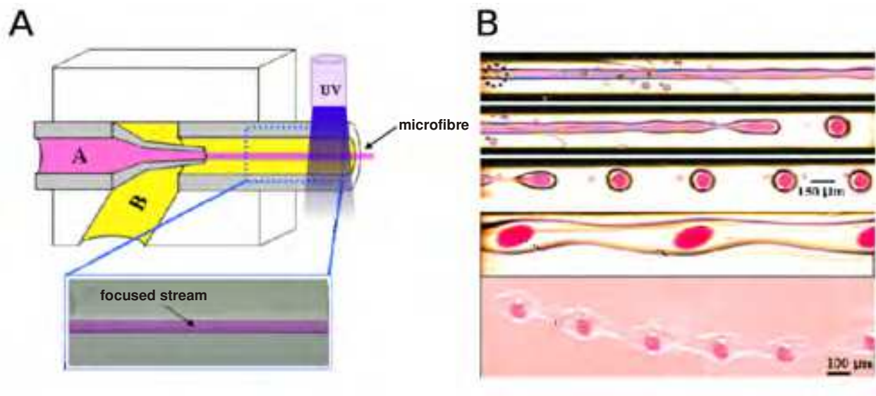
Fig. 4. Continuous fabrication of polymeric microfibres (Hyun et al., 2006; Jeong et al., 2004)
