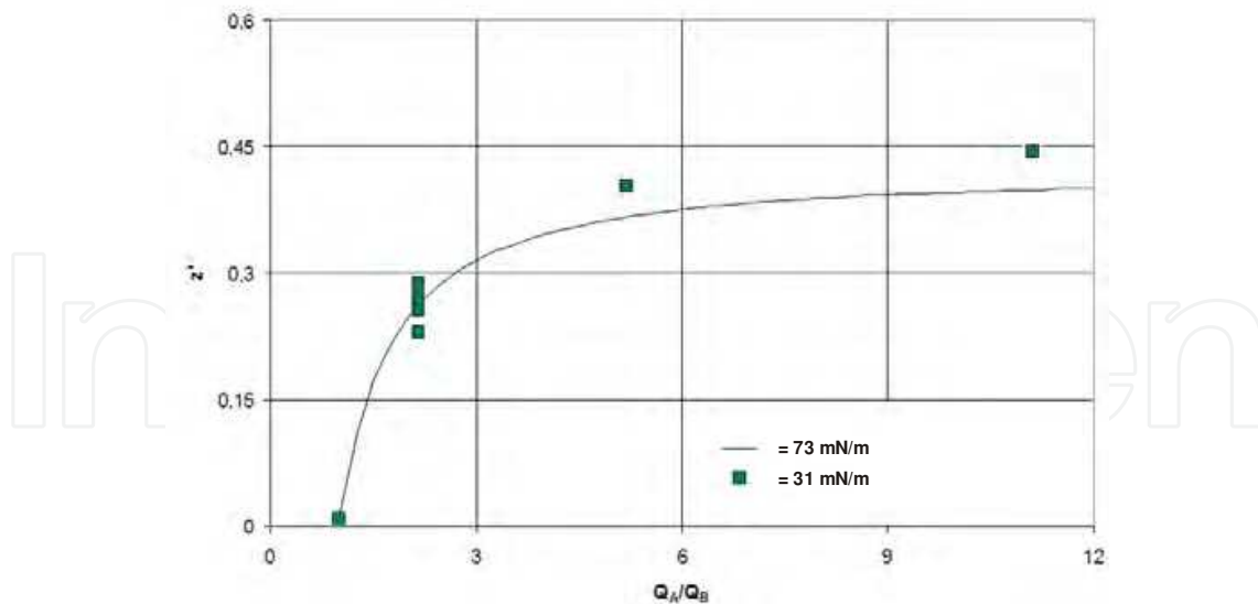
Fig. 18. The effect of surface tension of dimensionless stream curvature
