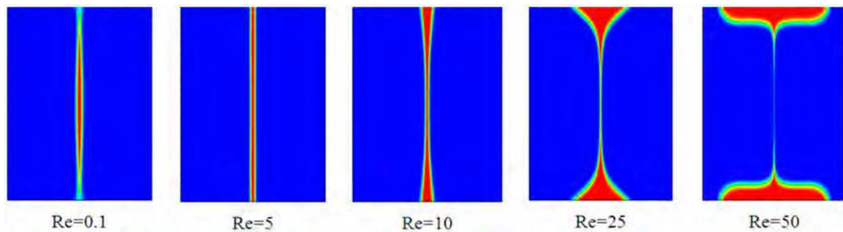
Fig. 8. Effect of Reynolds number on distributions of the focused liquid. Focusing ratio is 1:20 (Blonski et al.,2011)
