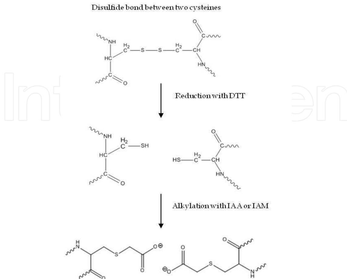
Fig. 3. The reduction and alkylation process: The breaking of disulfide bonds in proteins. Reduction by DTT to form cysteine residues must be followed by further modification of the reactive -SH groups (to prevent reformation of the disulfide bond) by acetylation by, in this case iodoacetic acid (adapted from (Nelson and Cox 2008)).
