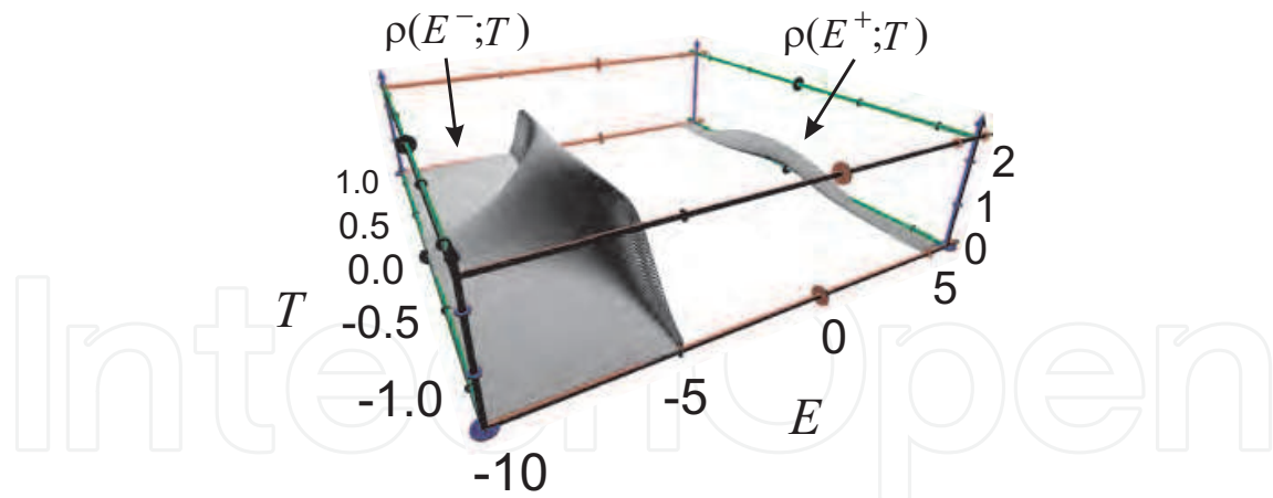
Fig. 10. Classical energy–time representation of a Gaussian density, centred at (q, p) = (0, -1) , for the nonlinear oscillator with a = 1, l = 2, k = 9.8, X = 0 , and \sigma = .8 . Dimensionless units.
