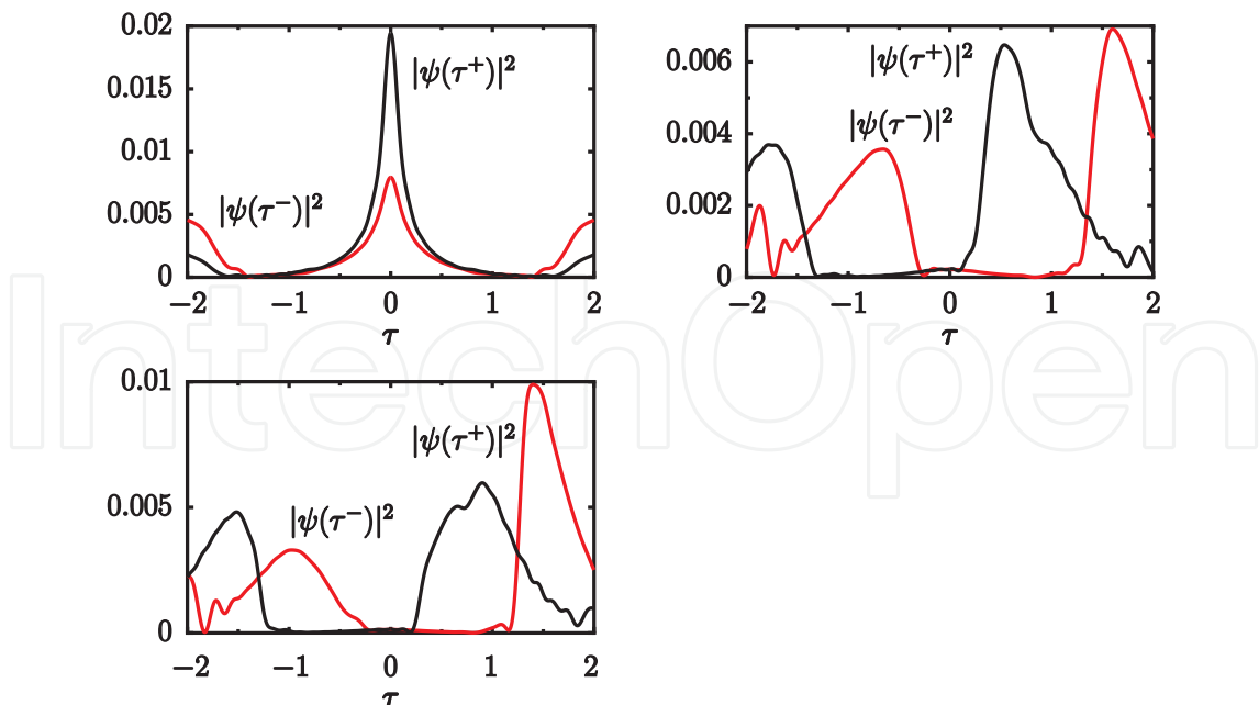
Fig. 9. Quantum time representation of the Gaussian state e^{-(q-q_0)^2/4\sigma^2 - ip_0(q-q_0/2)} / \sqrt{\sigma\sqrt{2\pi}} centred at (q, p) = (0, -1) , with \sigma = 0.2 , and for the nonlinear oscillator. The zero-time reference state is located at (a) X = 0 , (b) X the location of the right fixed point, and (c) X = 2 . Dimensionless units.
