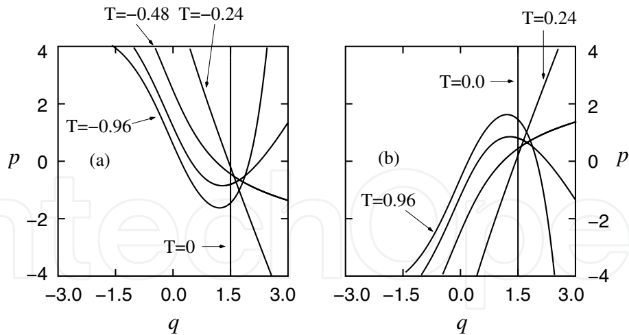
Fig. 3. Time surfaces for the nonlinear oscillator with a = 1 , l = 2 , and k = 9.8 . (a) Negative times and (b) positive times. The initial curve is q = 1.5 . Dimensionless units.
