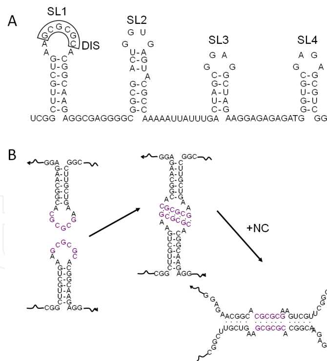
Fig. 3. Stem-loops of the HIV-1 5' untranslated region. (A) RNA structure of the four stem-loops. The dimerization initiation signal (DIS) sequence is shown in box. (B) Mechanism of viral RNA dimerization. Dimerization is initiated by base-pairing of the DIS forming a kissing-loop complex. Gag nucleocapsid (NC) promotes the formation of a more stable RNA dimer.
