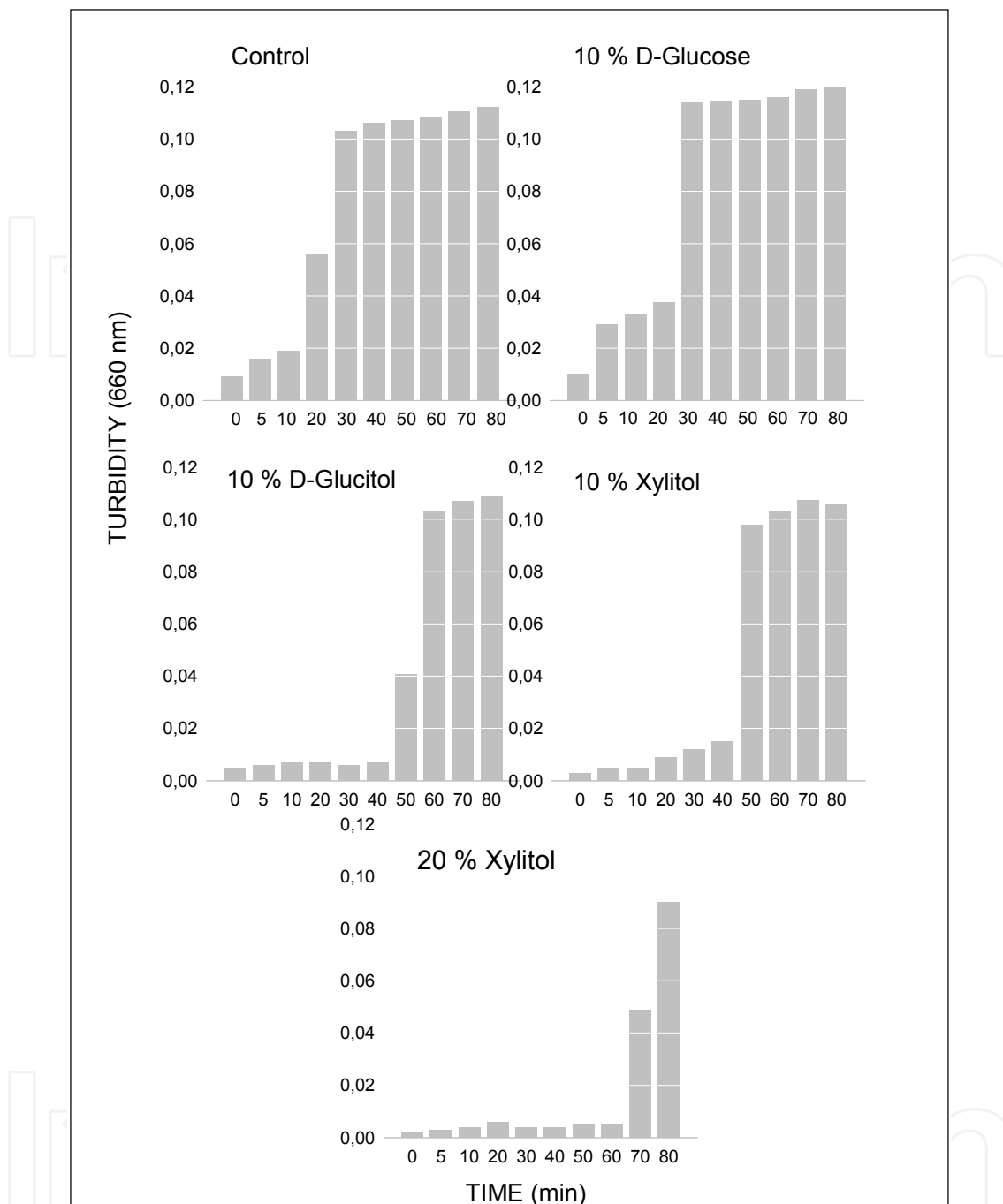
Fig. 2. An example of the stabilizing effect of alditols on the calcium phosphate system in an aqueous solution at pH 7.4. Inhibition by D-glucose, D-glucitol, and xylitol of Ca(II) phosphate precipitation at 37°C. The reactions were carried out using CaCl 2 as the source of Ca(II) and NaH 2 PO 4 as the source of phosphate (starting Ca(II) and phosphate concentrations were 2.40 mM and 1.44 mM, respectively). The formation of Ca(II) precipitates was monitored over a period of 80 min by measuring the turbidity of the mixtures at 660 nm. The procedures have in principle been described in Mäkinen & Söderling, 1984
